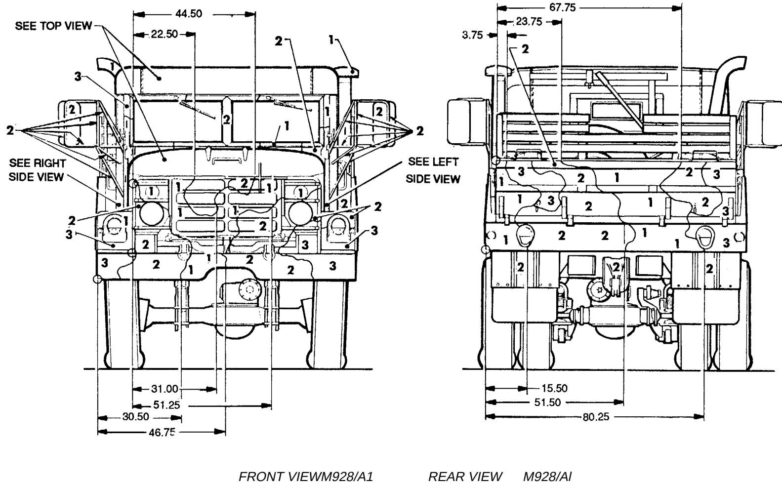
Figure 69. Truck, cargo: 5-ton, XLWB, M927A1 and M928A1. (1 of 4)
