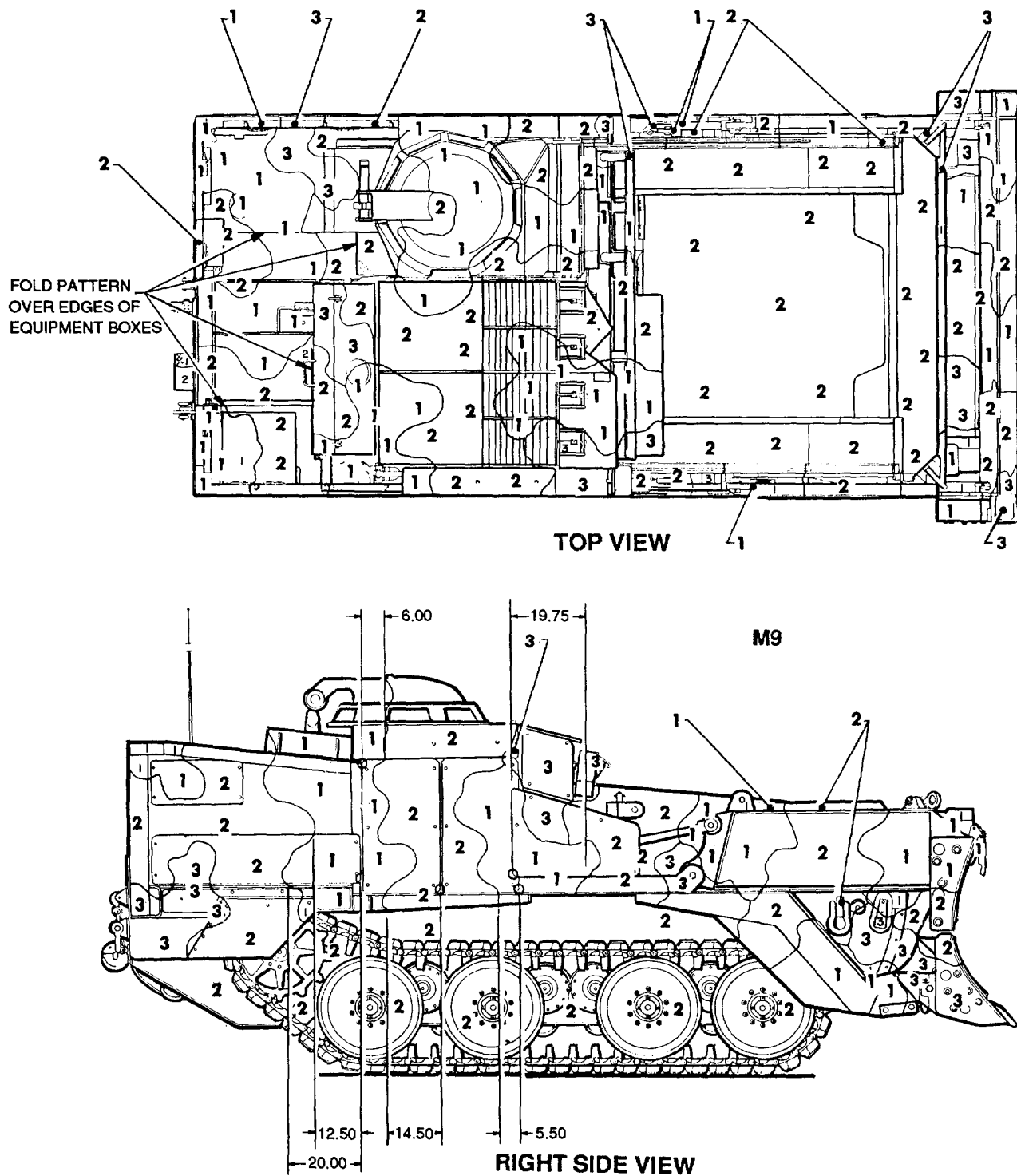
Figure 161. Earthmover, armored, combat, M9. (1 of 2)
