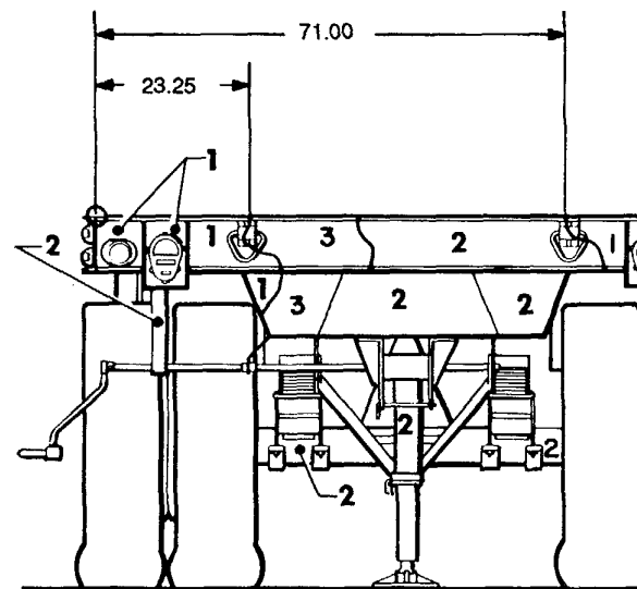
REAR VIEW
