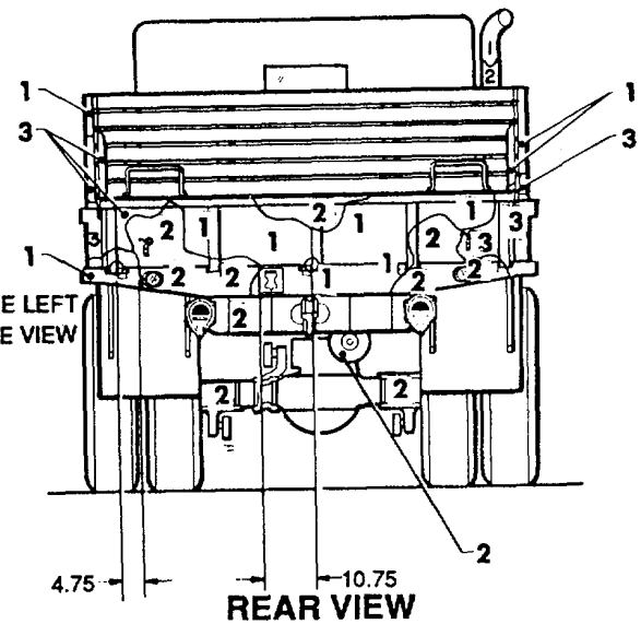
Figure 47. Truck, cargo/personnel: 6 x 6, 2-1/2-ton, M35A2, M35A2C, and V18A. (1 of 2)
