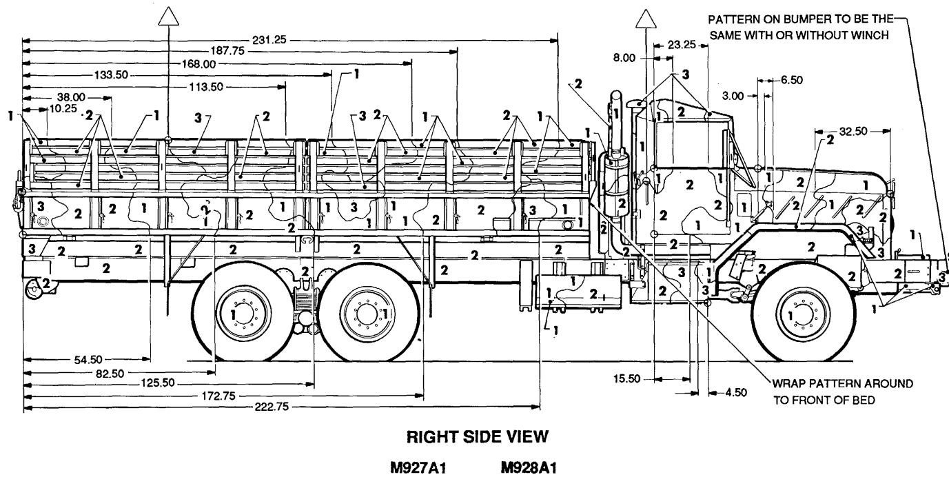
Figure 69. Truck, cargo: 5-ton, XLWB, M927A1 and M928A1. (4 of 4)
