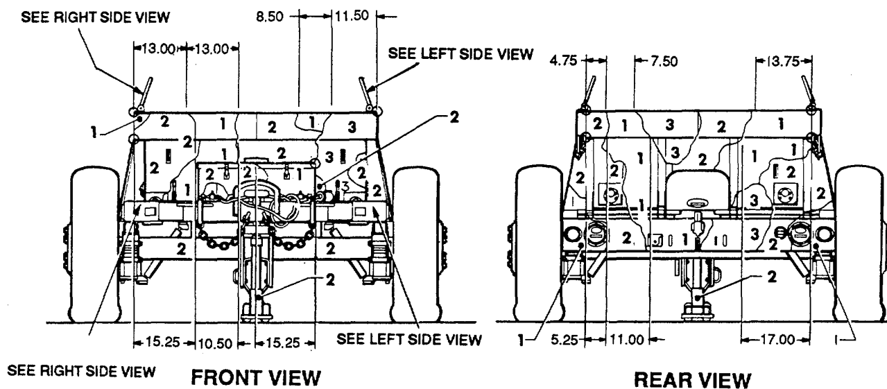
Figure 127. Trailer, ammunition: 1-1/2-ton, 2-wheel, M332. (2 of 2)
