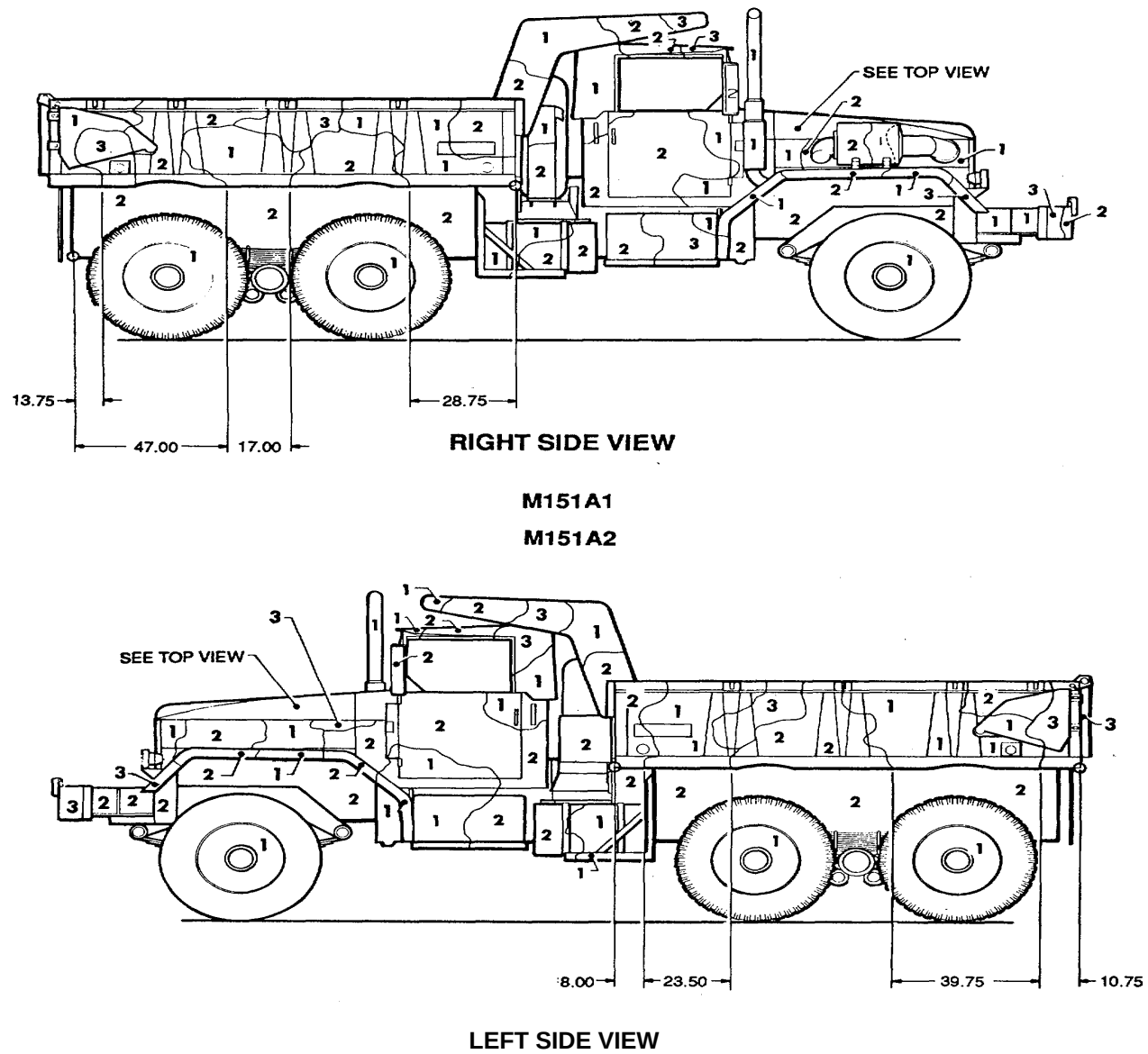
Figure 56. Truck, dump: 5-ton, w/winch, M151A1 and M151A2. (2 of 2)
