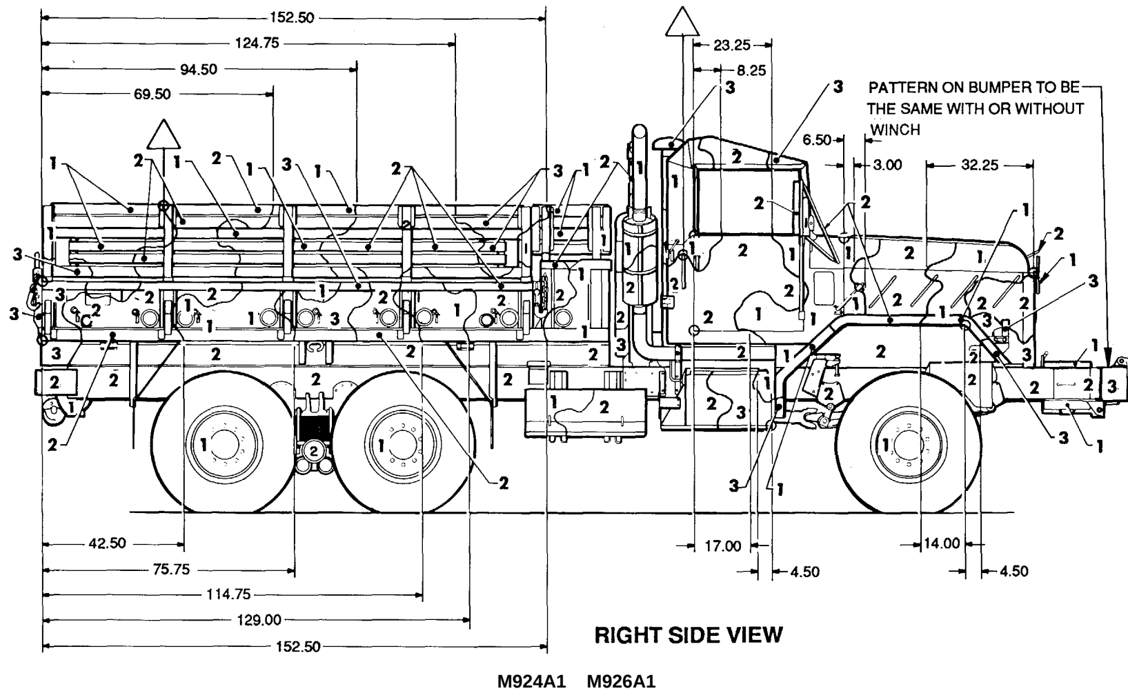
Figure 68. Truck, cargo: 5-ton, M924A1 and M926A1. (4 of 4)
