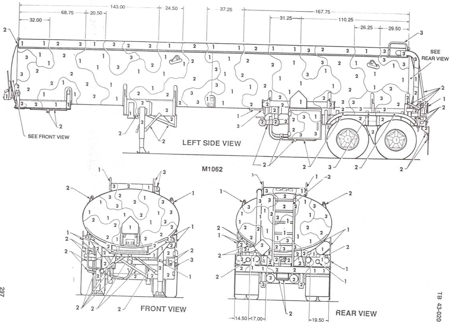
Figure 141. Semitrailer, tanker: 7500 gallon, M1062. (2 of 2)
