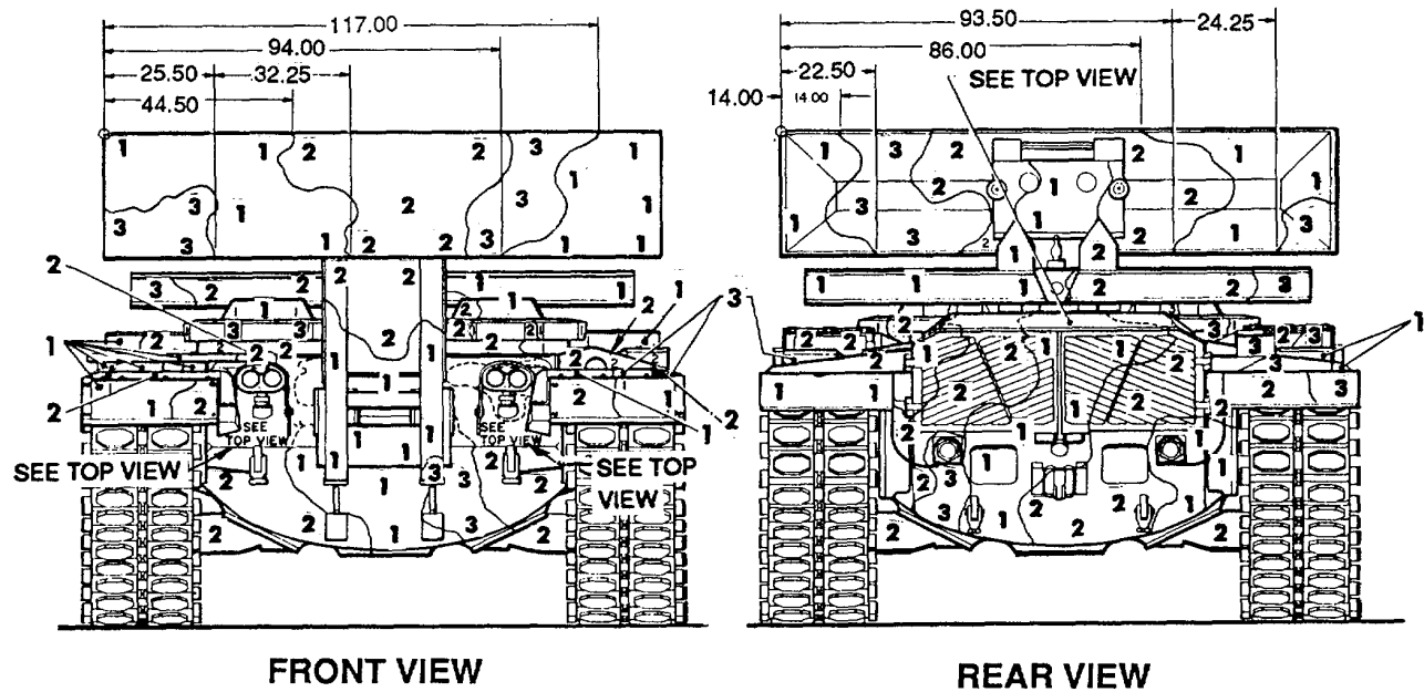
Figure 96. Launcher and M48A5 tank chassis, transporting for Bridge, armored-vehicle-launched scissoring type, class 60. (2 of 2)
