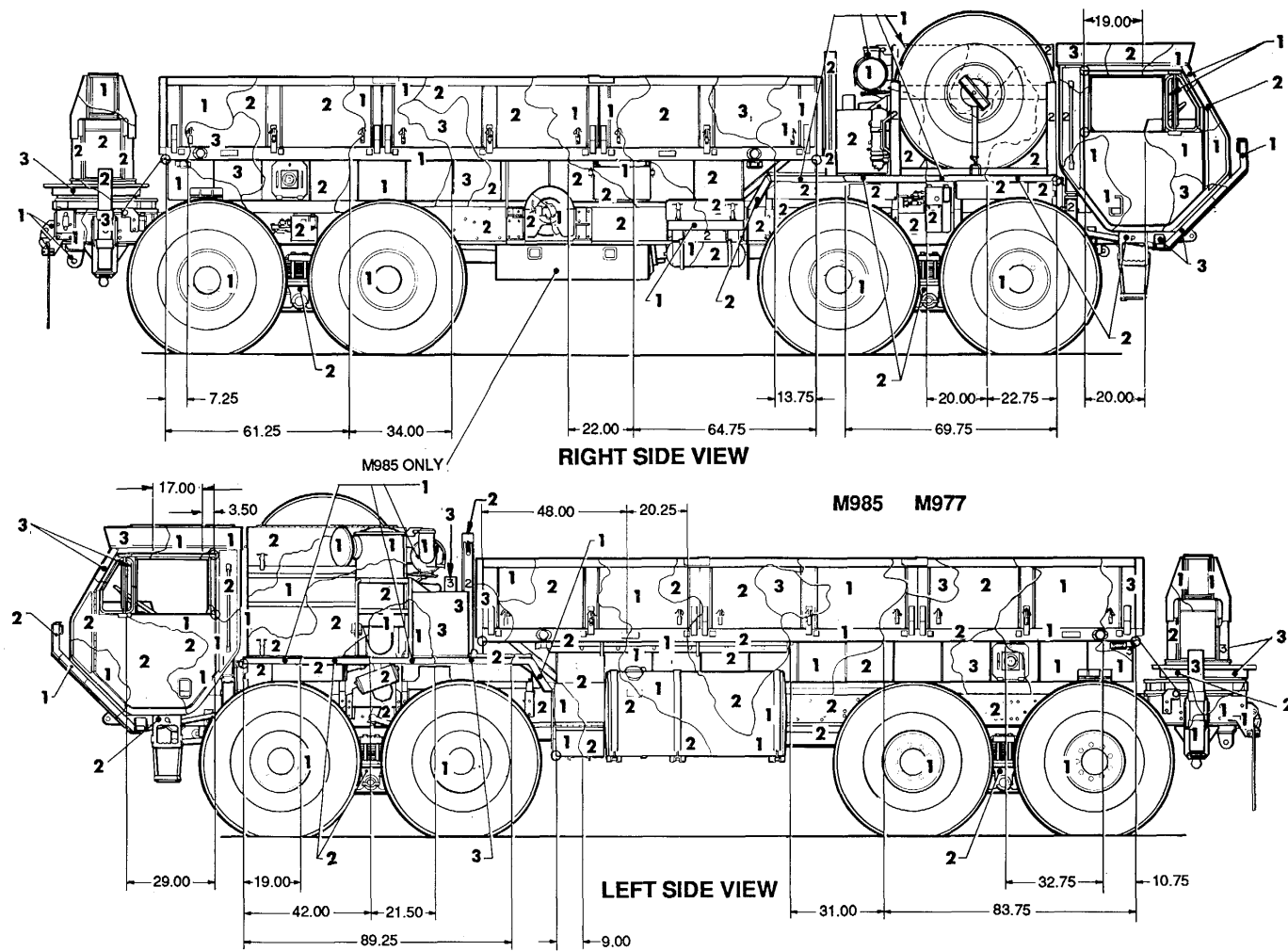
Figure 86. Truck, cargo: 11-ton, M977 and M985. (2 of 2)
