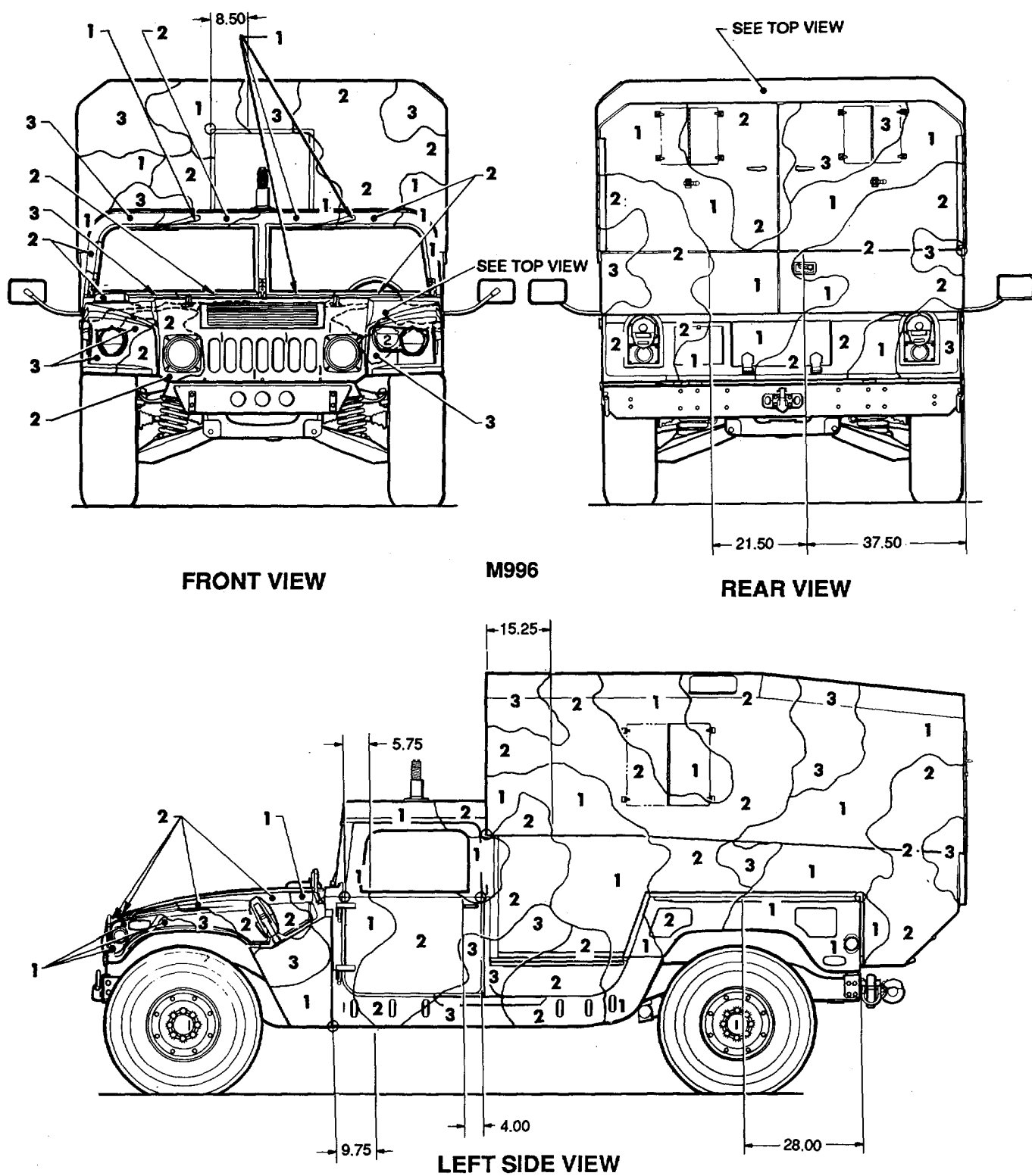
Figure 38. Ambulance, 2-liter, hard top, 4 x 4, M996. (2 of 2)
