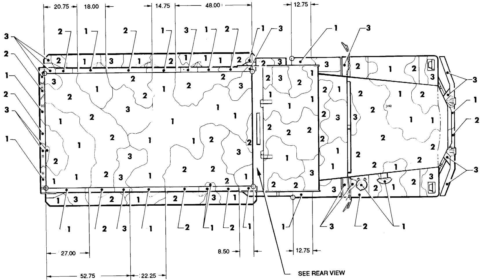
TOP VIEW
