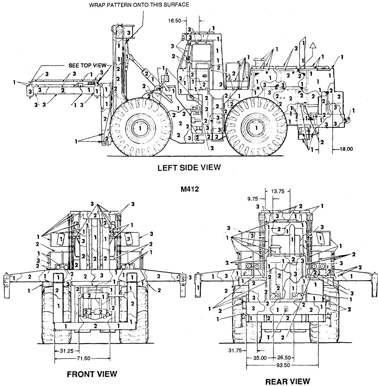
Figure 173. Loader, RT container handler, M412. (2 of 2)
