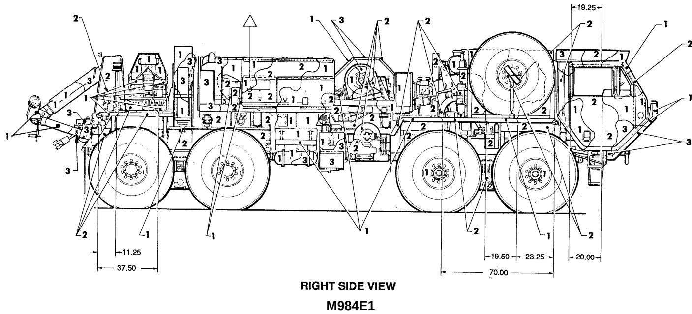
Figure 85. Truck, wrecker: 11-ton, M984E1. (4 of 4)
