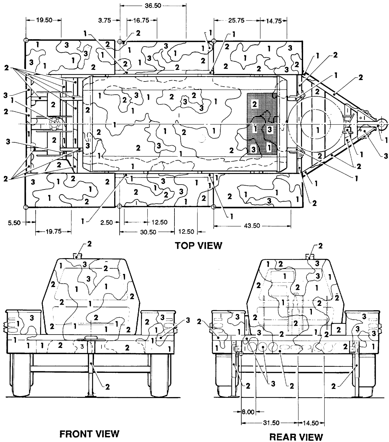
Figure 151. Air compressor: 250-CFM. (1 of 2)
