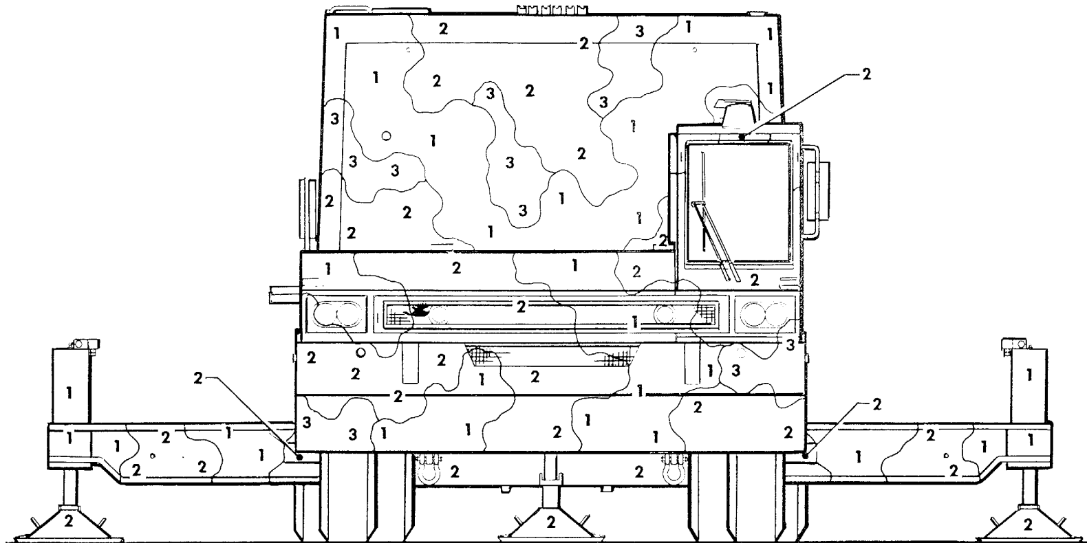
FRONT VIEW
