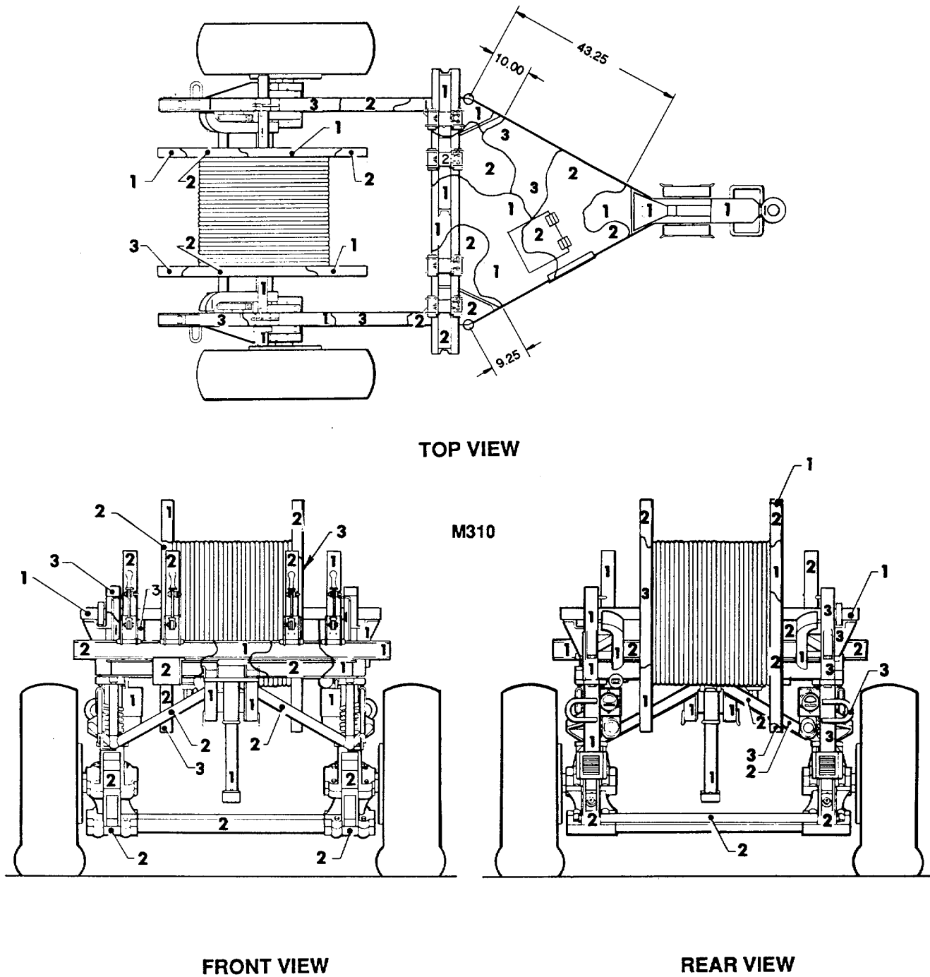
Figure 126. Trailer, cable reel: M310. (1 of 2)
