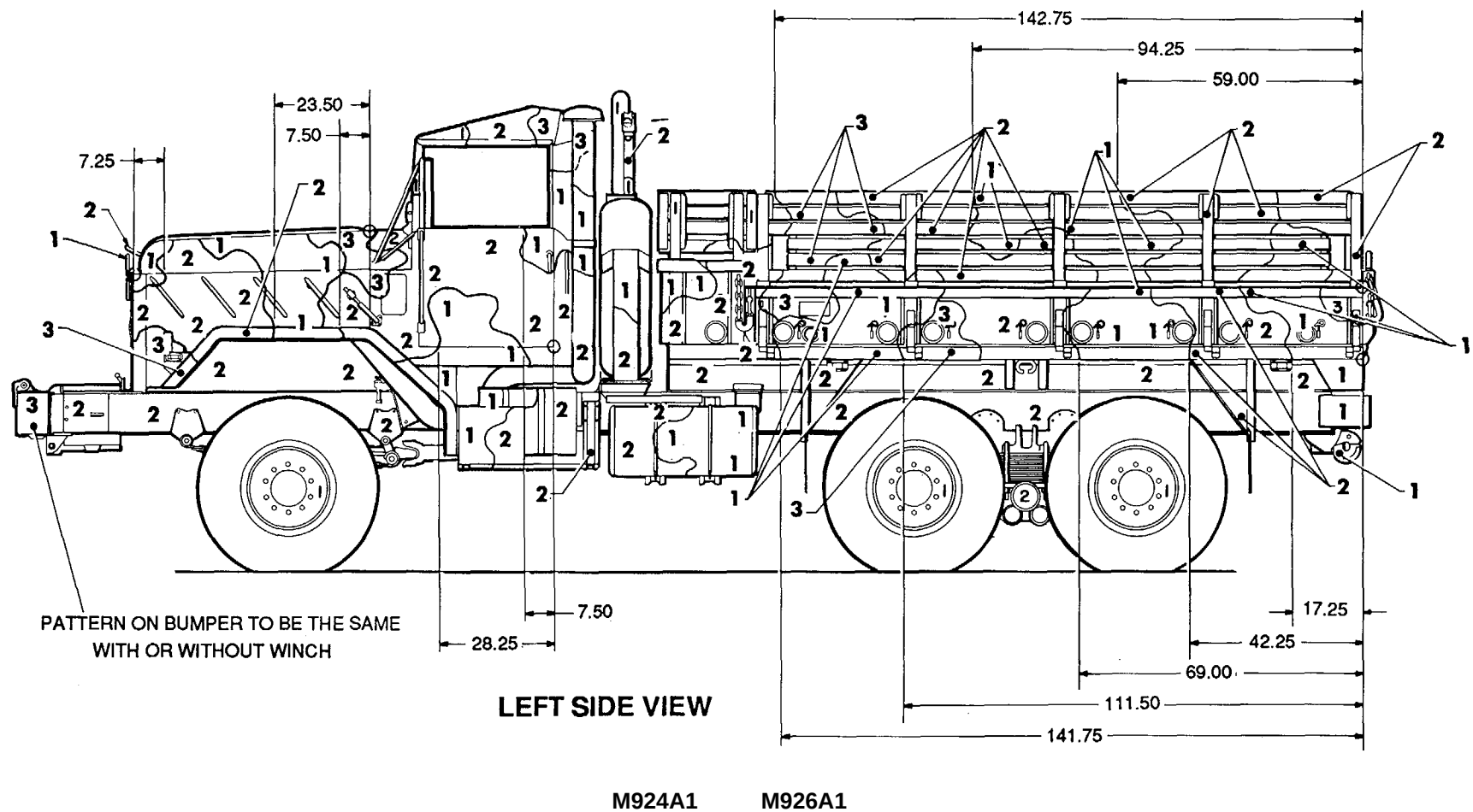
Figure 68. Truck, cargo: 5-ton, M924A1 and M926A1. (2 of 4)
