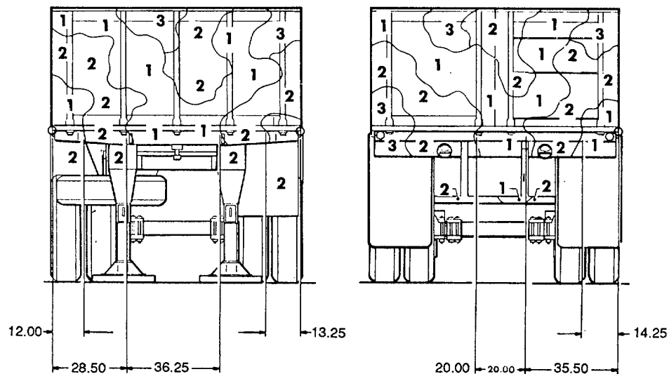
FRONT VIEW
