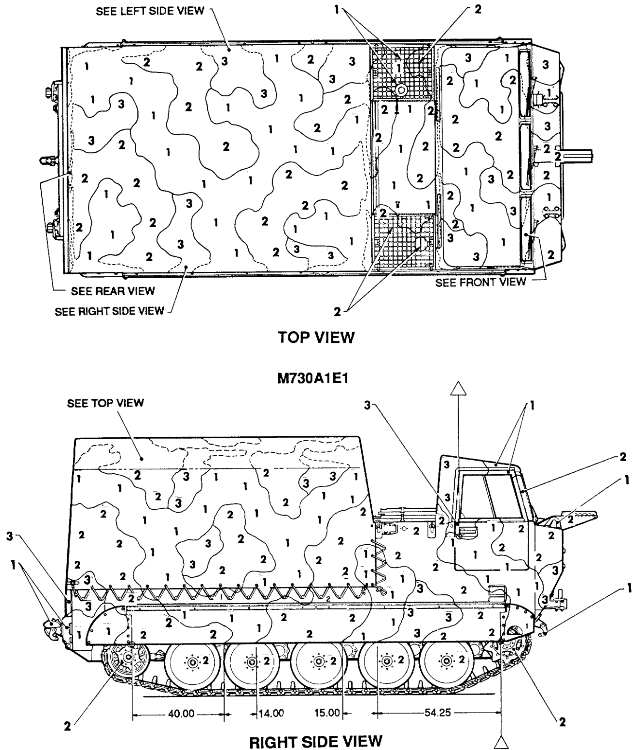
Figure 116. Carrier, guided missile equipment, M730A1E1. (1 of 2)
