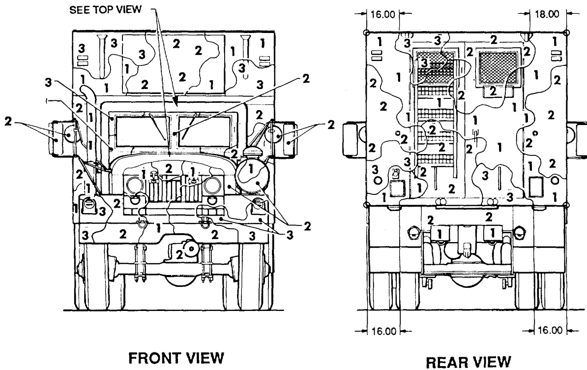
Figure 65. Truck, van, expansive: 5-ton, M820A2. (1 of 2)
