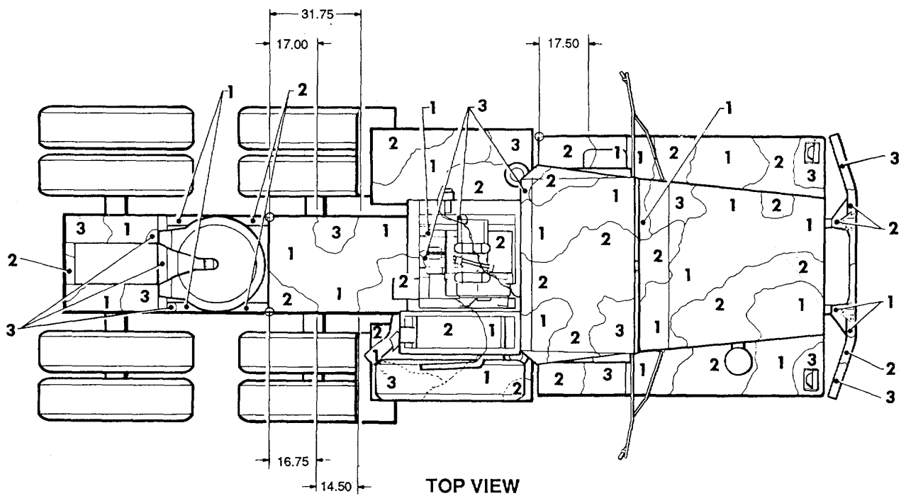
Figure 76. Truck, tractor: 10-ton, M123A2C, wolwhich. (1 of 2) 150
