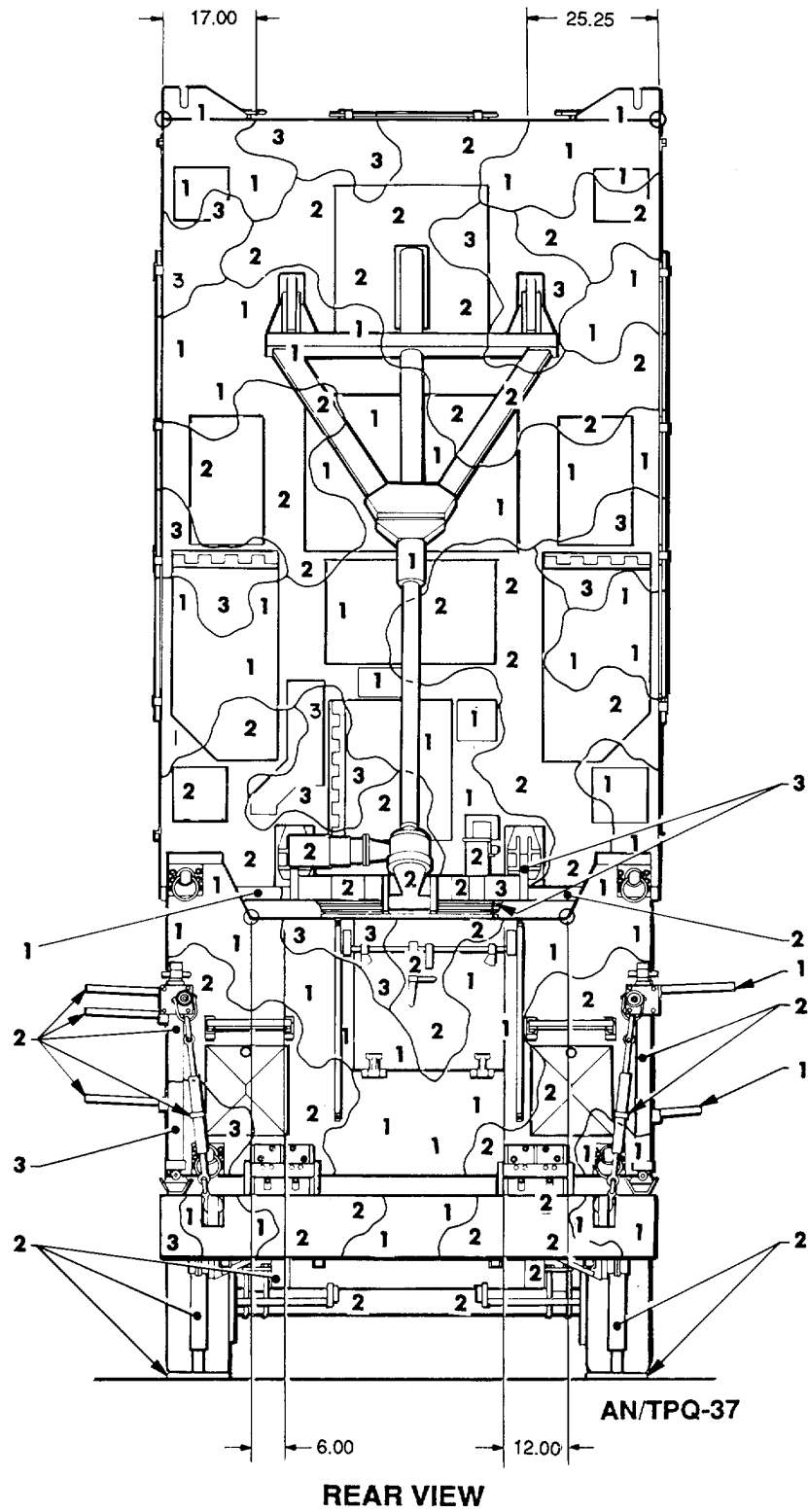
Figure 165. Trailer, chassis: antenna transceiver group, AN/TPQ-37. (4 of 5)
