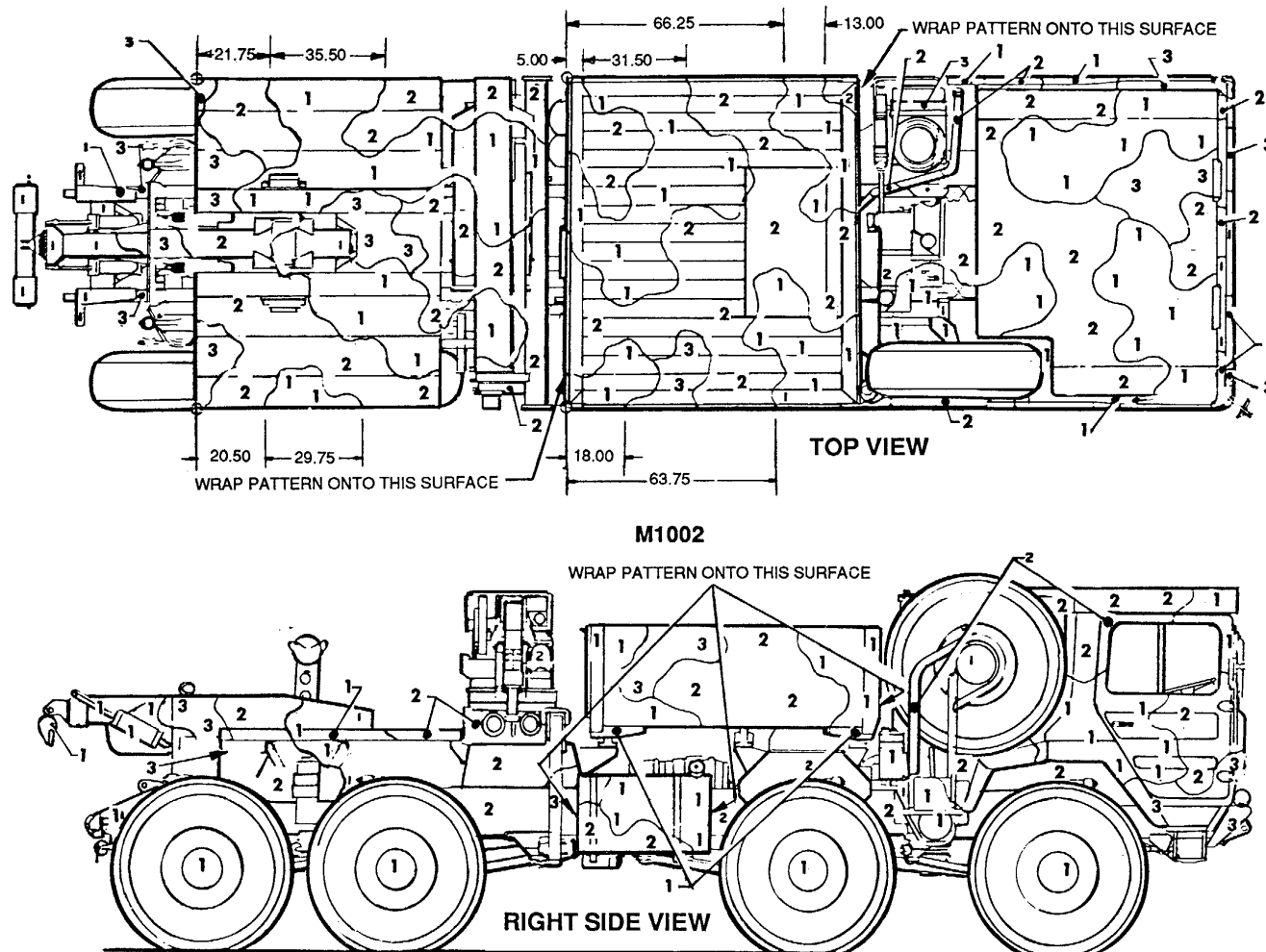
Figure 79. Truck, wrecker: 10-ton, M1002. (1 of 2)
