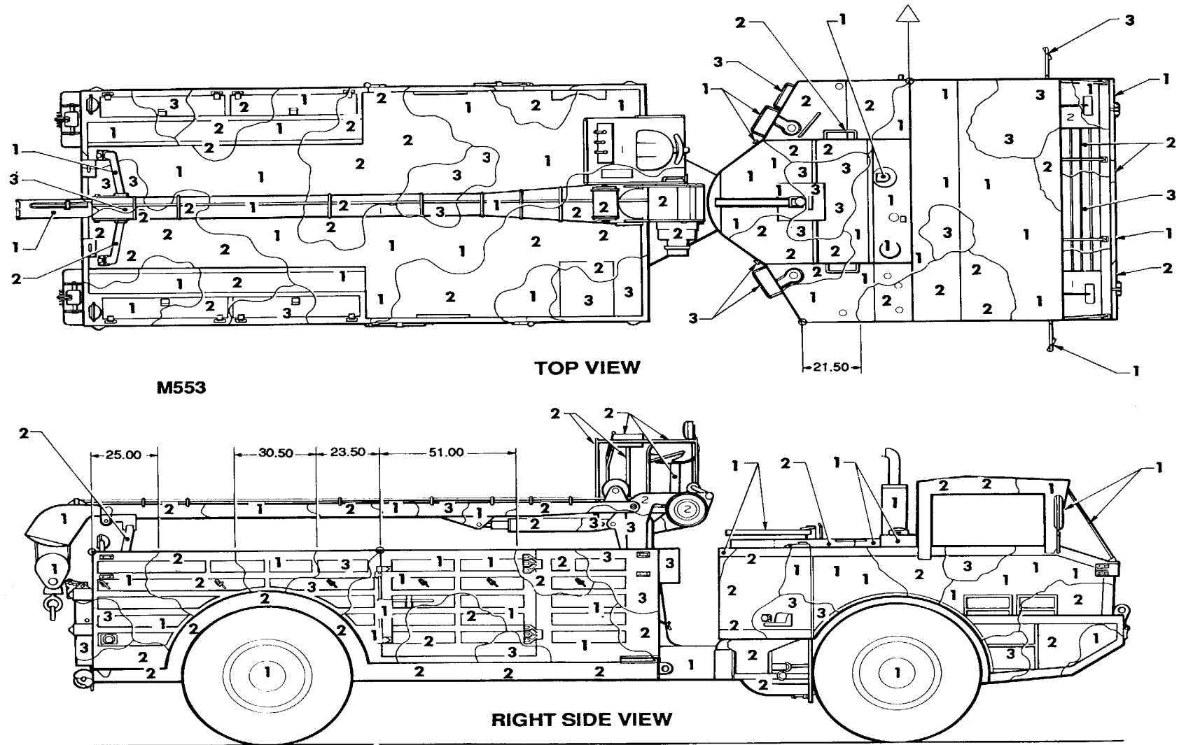
Figure 64. Truck, wrecker: 10-ton, 4 x 4, M553. (2 of 2)
