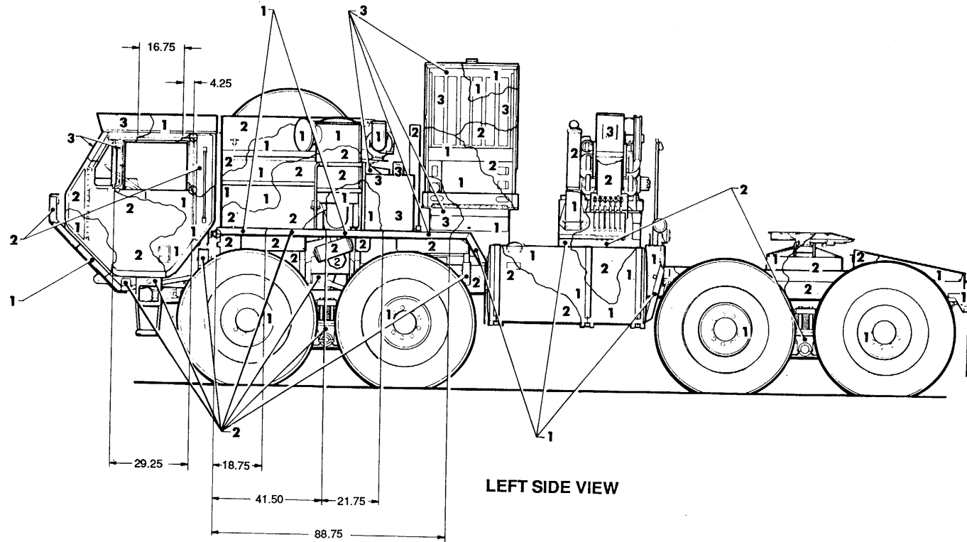
M983 W/CRANE
