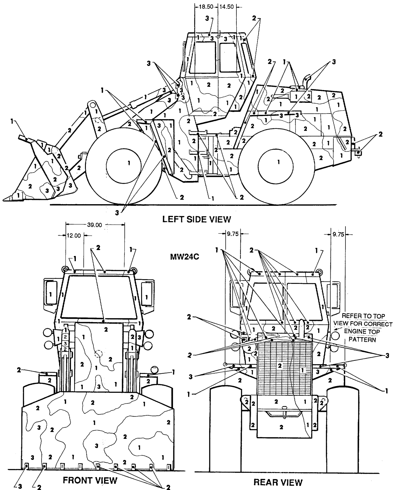
Figure 163. Scoop loader, 2-1/2 CY, MW24C. (2 of 2)
