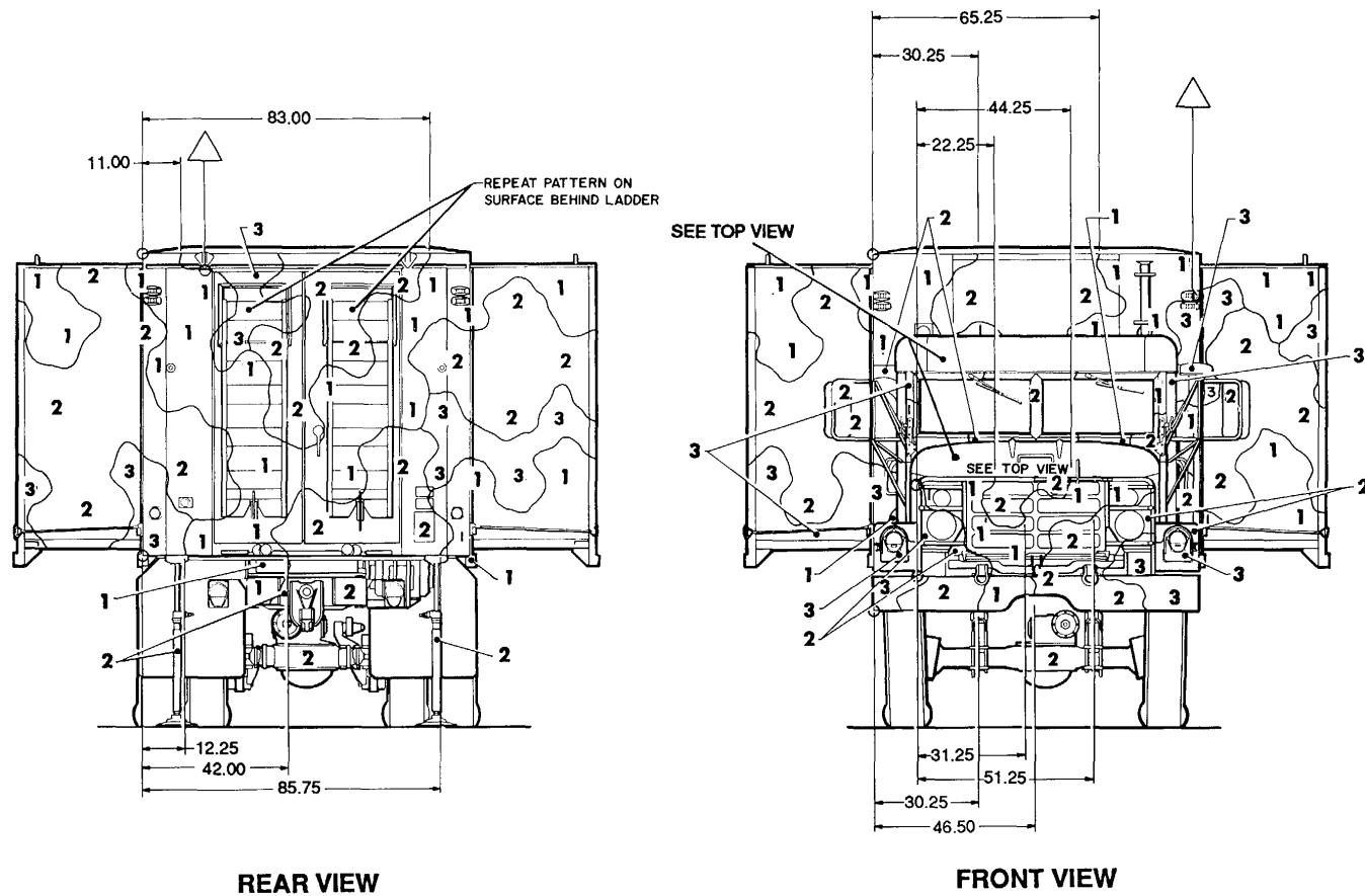
Figure 72. Truck, van, expensible: 5-ton, M934A1 and M935A1. (1 of 4)
