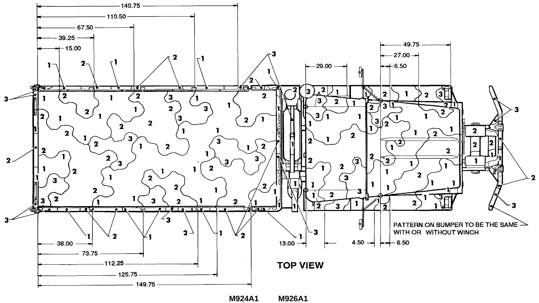
Figure 68. Truck, cargo: 5-ton, M924A1 and M926A1. (3 of 4)
