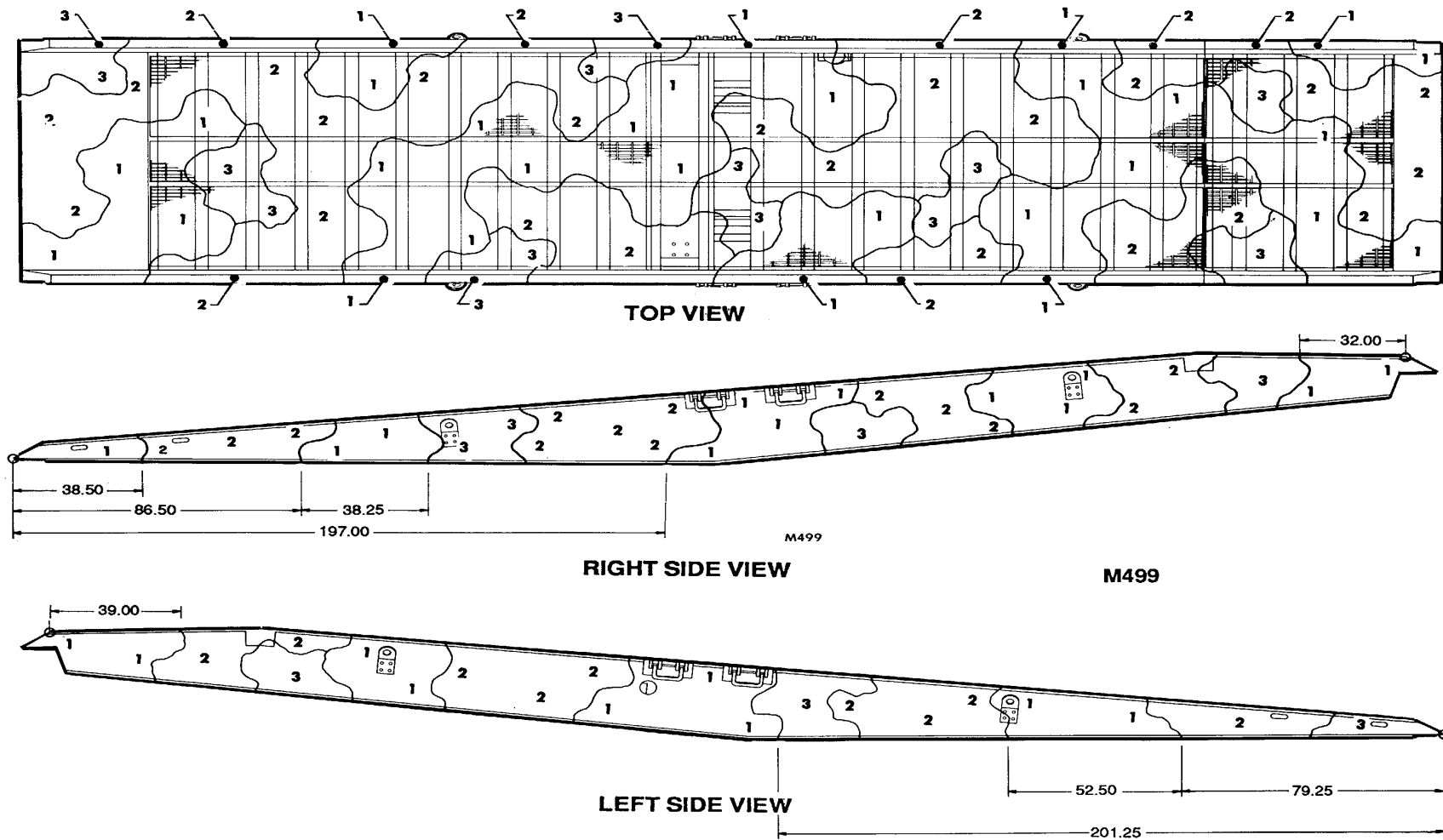
Figure 166. Ramp, M499.
