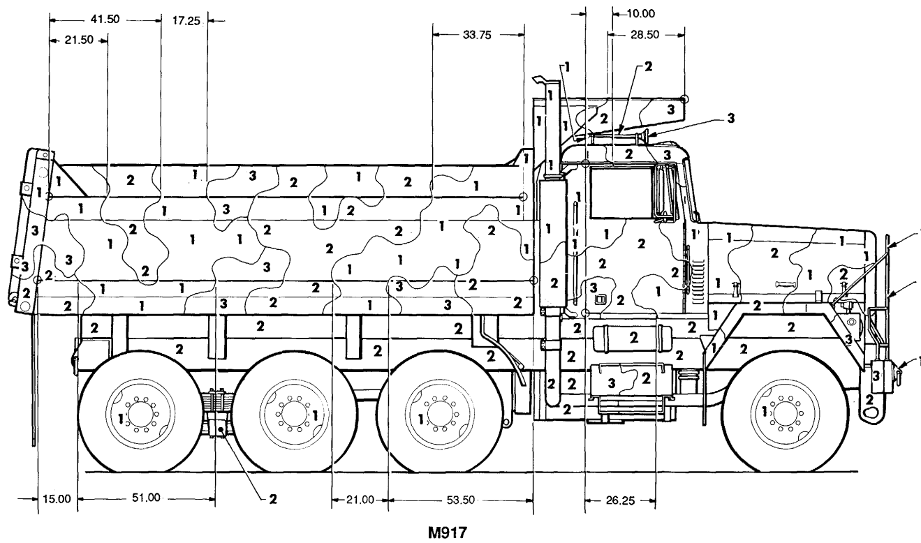
Figure 88. Truck, dump: 20-ton, M917. (2 of 4)
