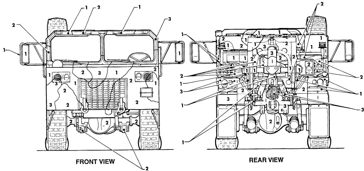
M984E1
