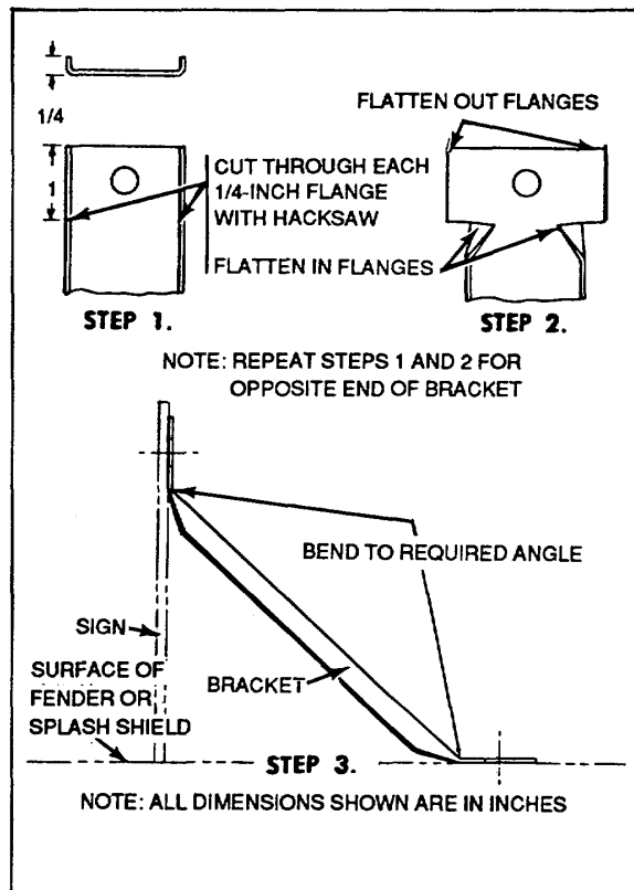
Figure 24. Alteration of bracket.
