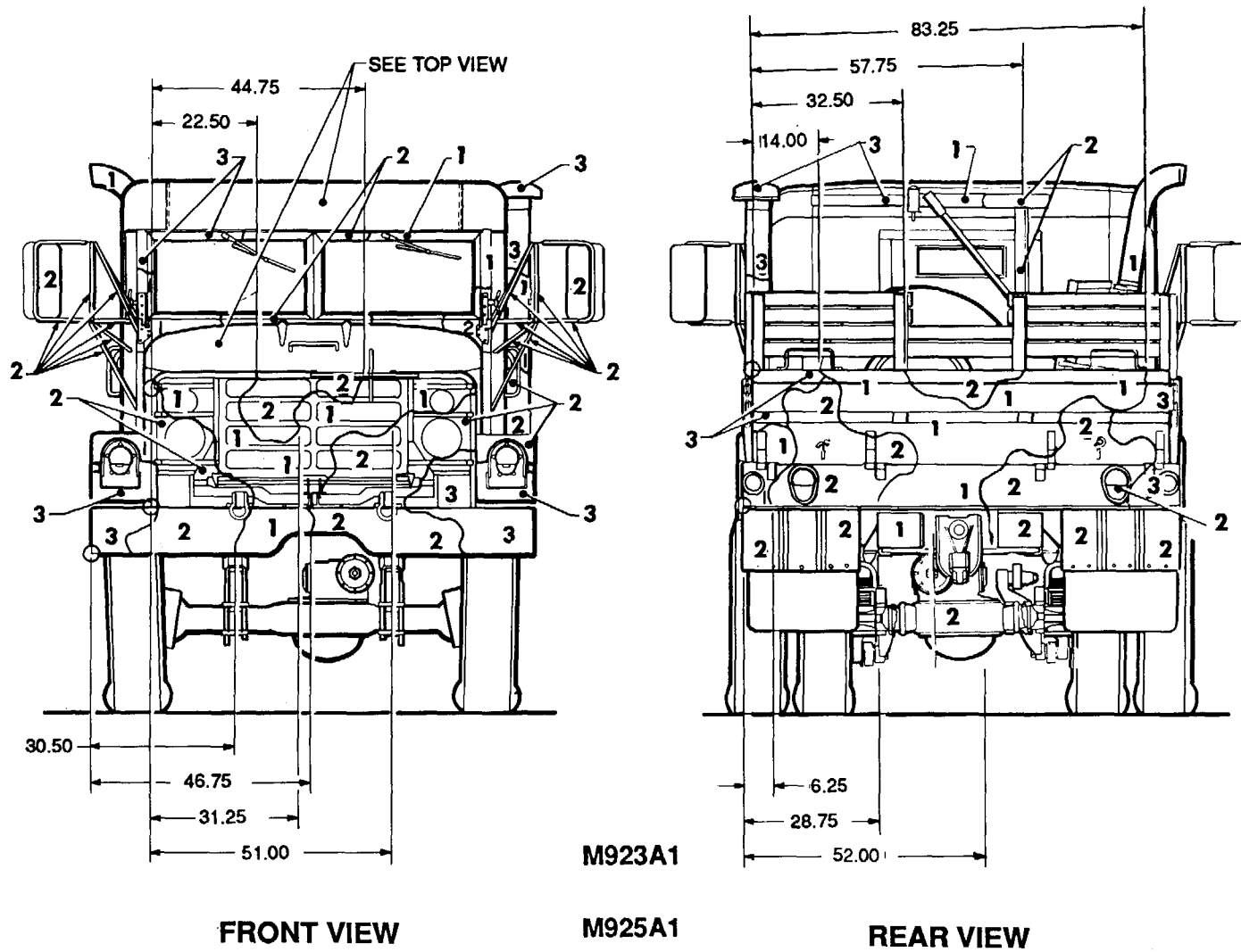
Figure 67. Truck, cargo: 5-ton, M923A1 and M925A1. (1 of 4)
