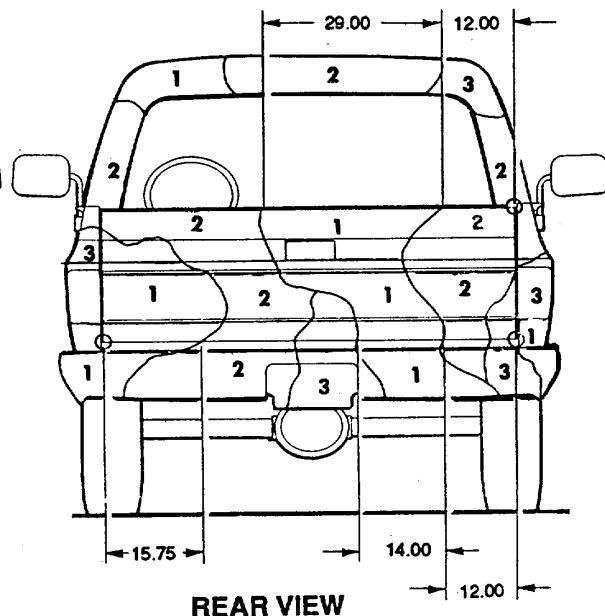
Figure 44. Truck, utility: 3/4-ton, 4 x 4, M1009. (1 of 2)
