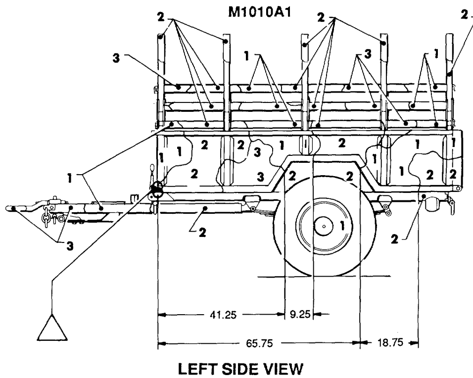
Figure 122. Trailer, cargo: 3/4-ton, 2-wheel, M101A1. (2 of 2)
