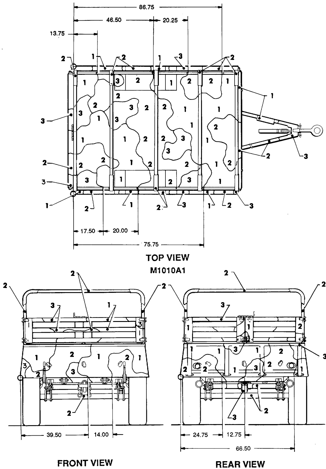
Figure 122. Trailer, cargo: 3/4-ton, 2-wheel, M101A1. (1 of 2)
