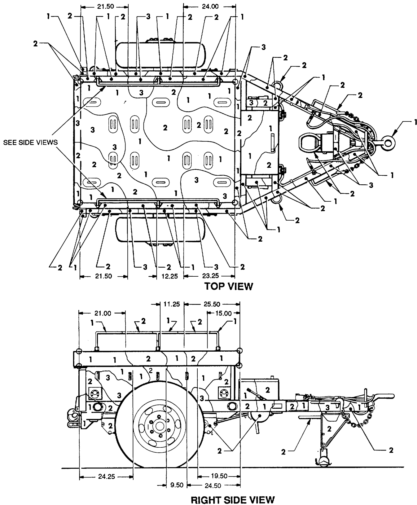
Figure 127. Trailer, ammunition: 1-1/2-ton, 2-wheel, M332. (1 of 2)
