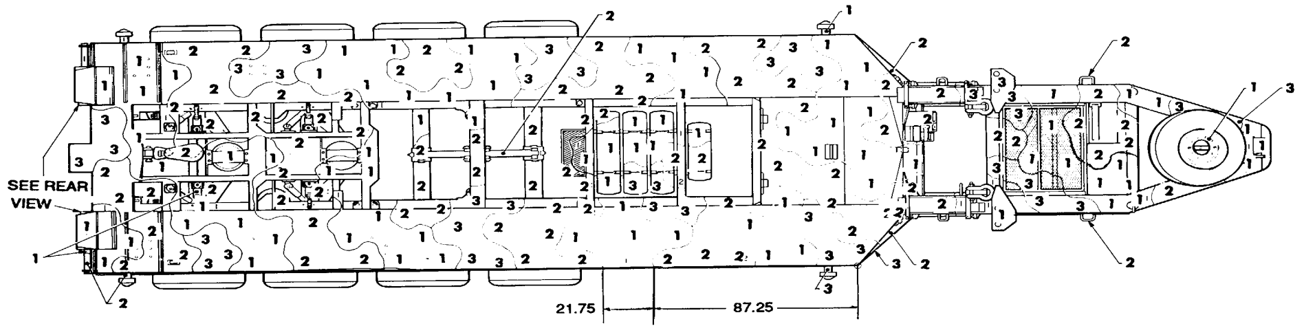
TOP VIEW
