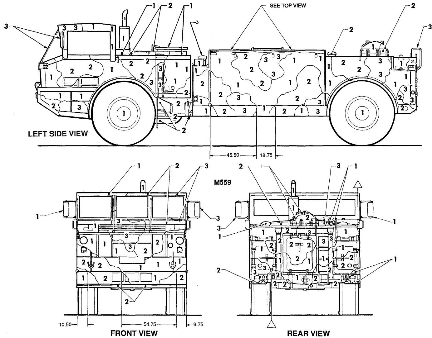
Figure 75. Truck, tank: fuel servicing, 2500 gallon, 4 x 4, M559. (2 of 2)
