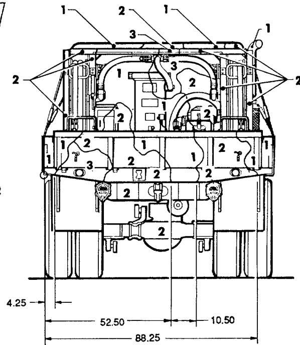
Figure 48. Truck, distribution, fuel/water: 6 x 6, 2-1/2-ton series. (1 of 2)
