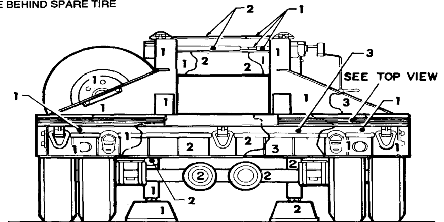
REAR VIEW
