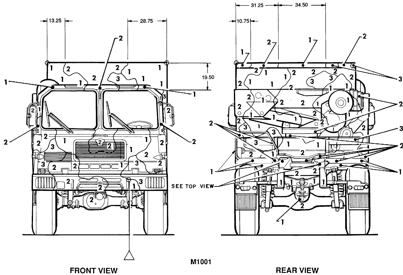
Figure 78. Truck, tractor: 10-ton, M001. (1 of 4)
