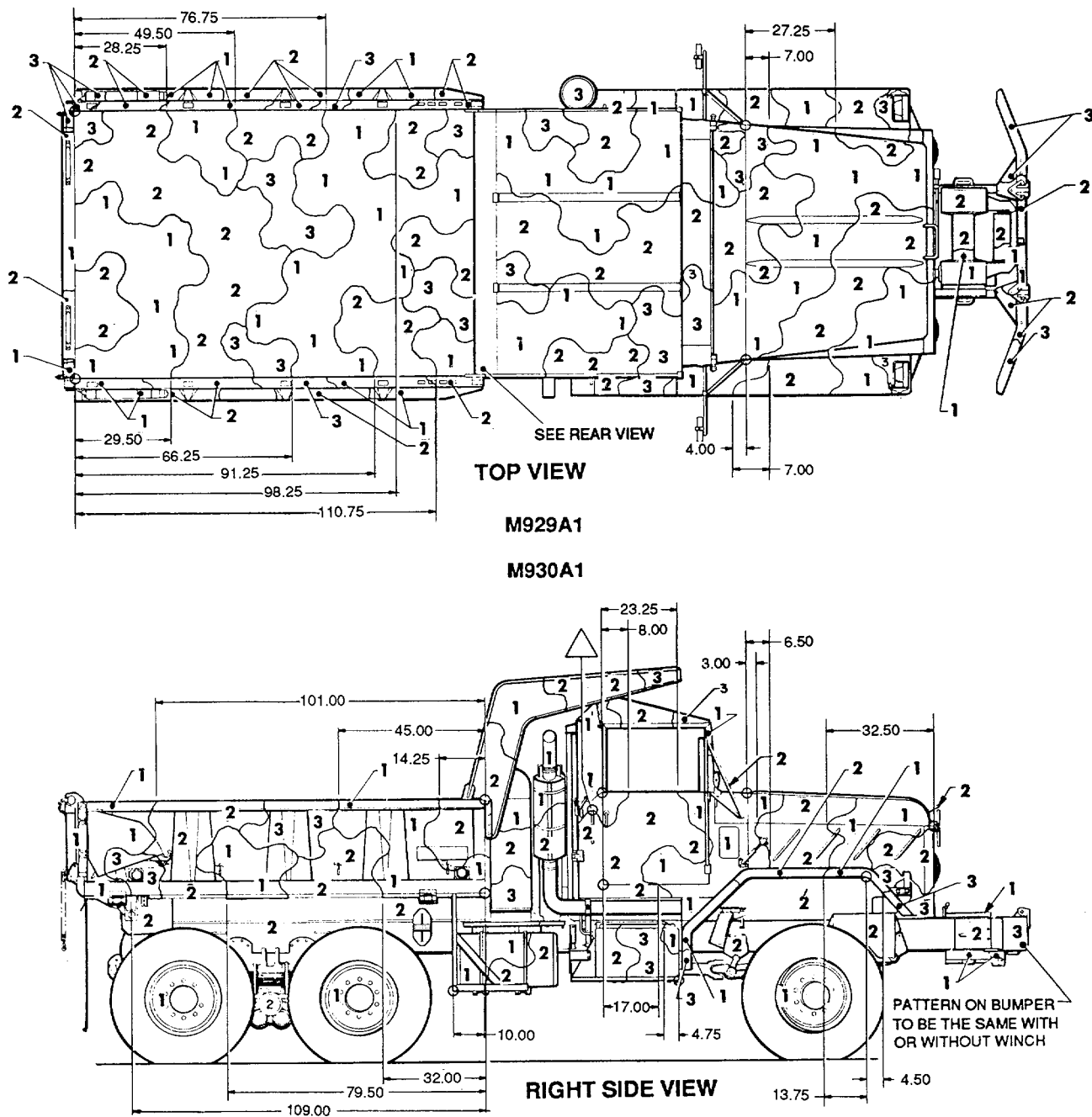
Figure 70. Truck, dump: 5-ton, M929A1 and M930A1. (1 of 2)
