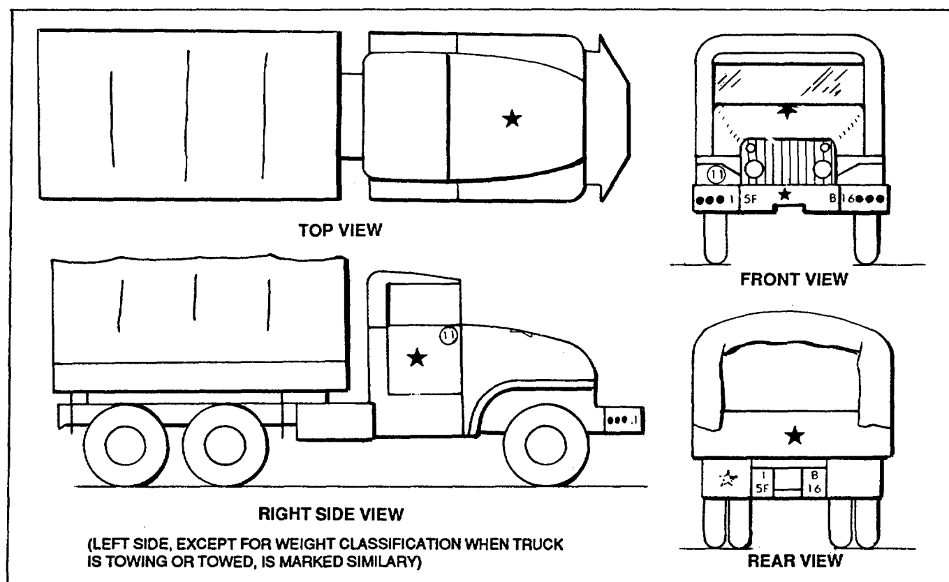
Figure 5. Marking locations—(typical) 2-1/2-, 5- and 10-ton trucks.
