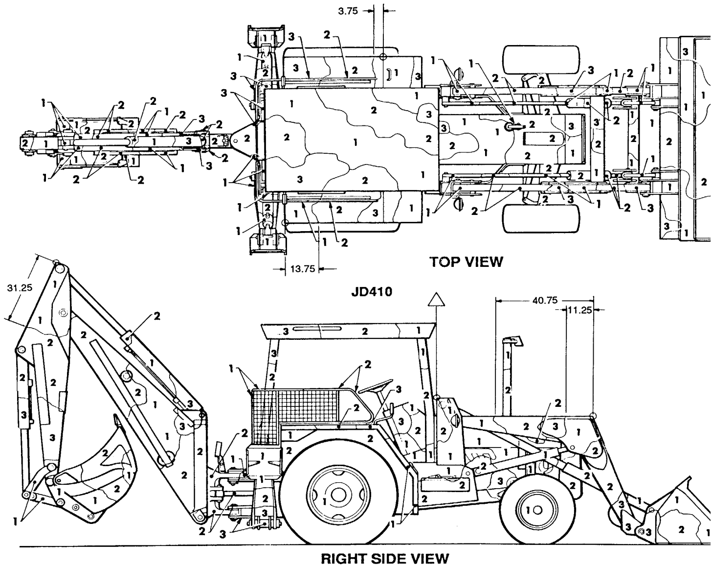
Figure 156. Tractor, wheeled, DED, w/backhoe, w/front loader, JD-140. (1 of 2)
