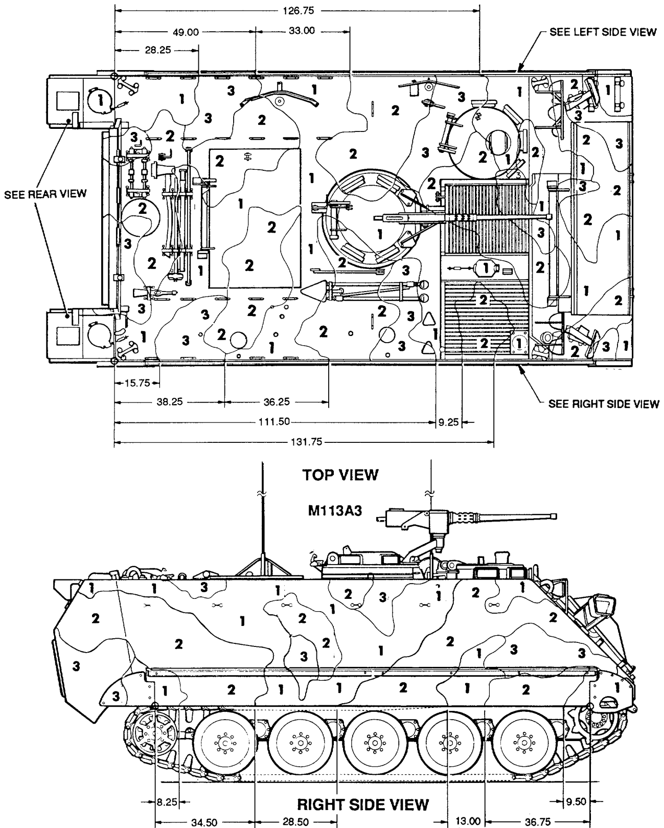
Figure 108. Carrier, personnel: M113A3. (1 of 2)
