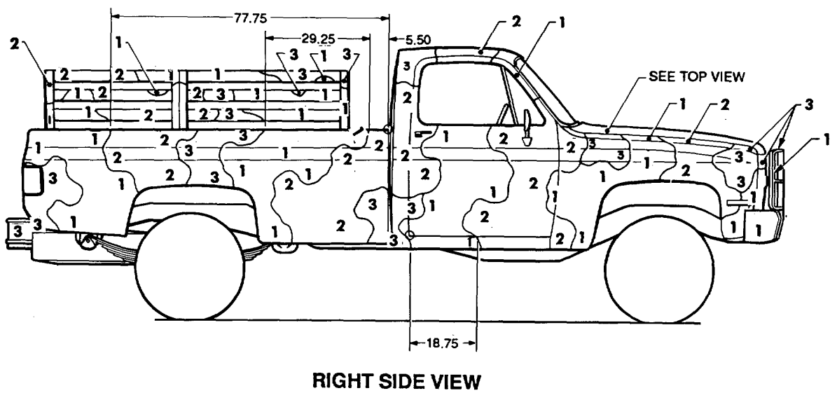
Figure 43a. Truck, cargo: 1-1/4-ton, 4 x4, M1008. (1 of 2)
