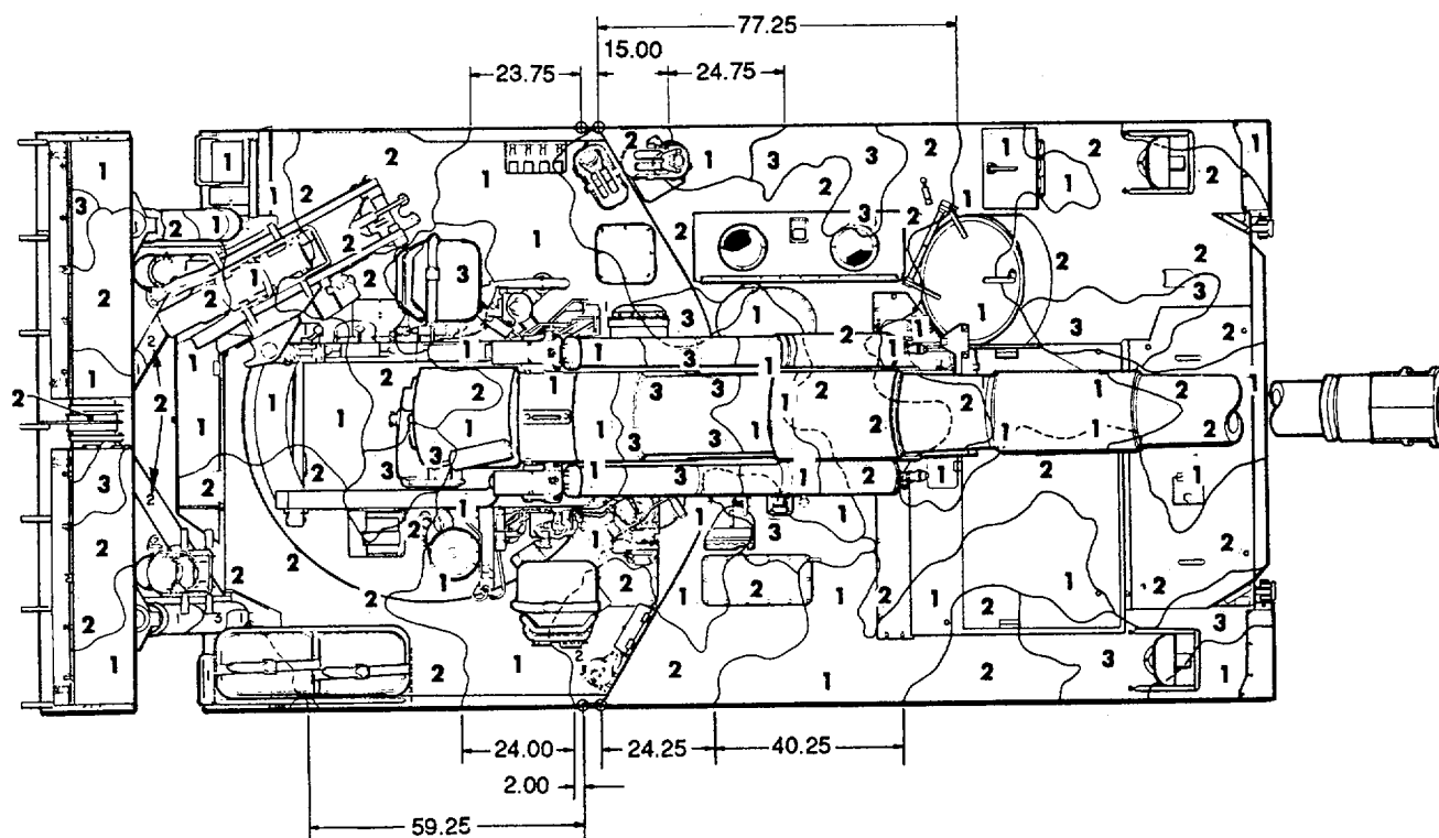
TOP VIEW
