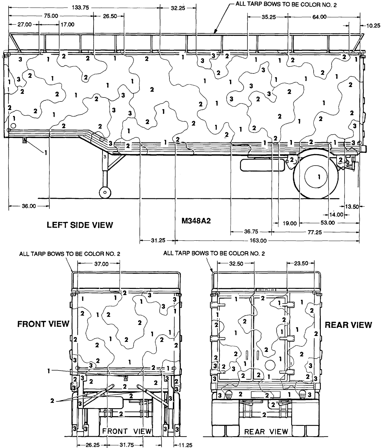
Figure 137. Semitrailer, van: composite, 6-ton, 2-wheel, M348A2. (2 of 2)
