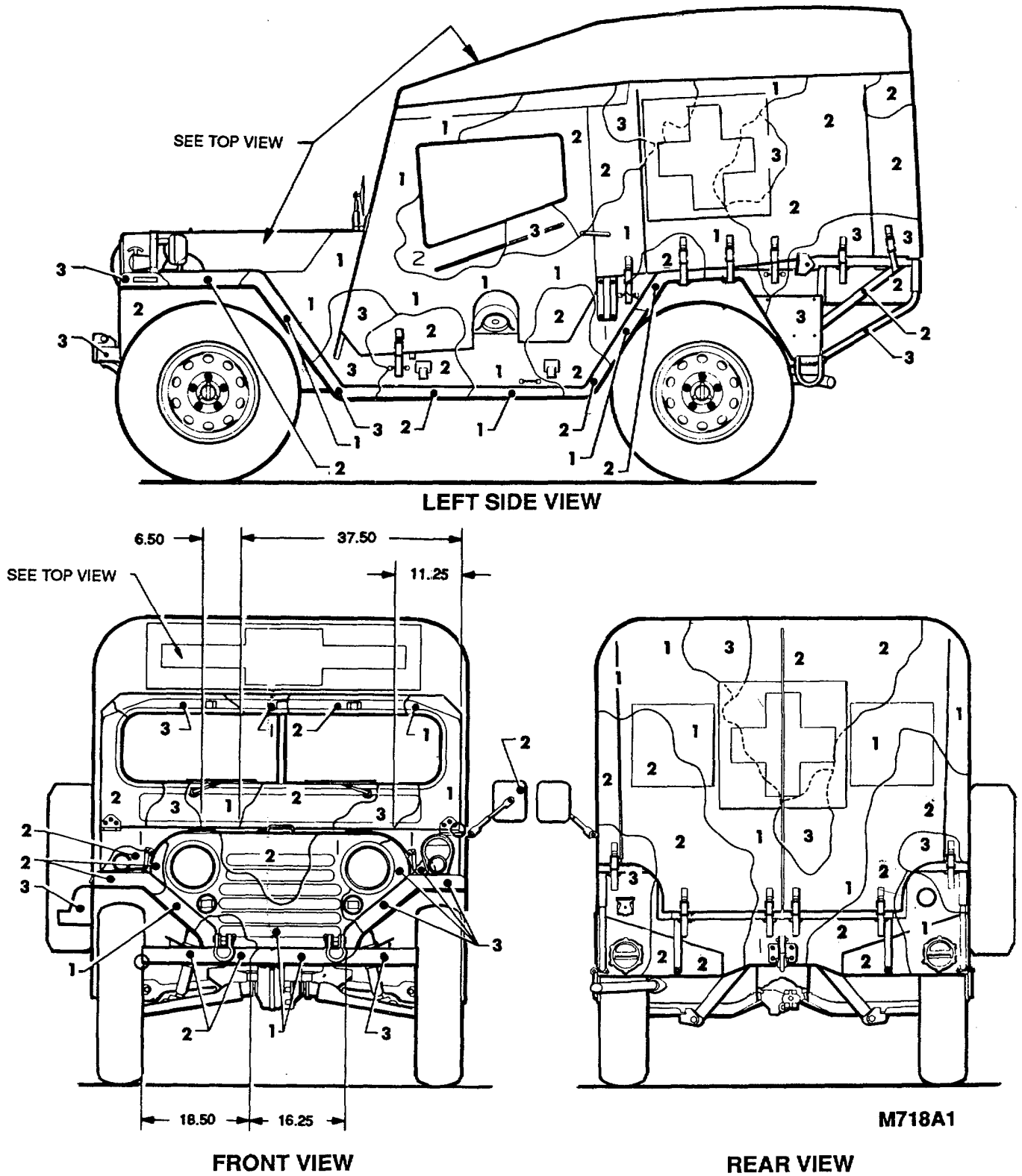
Figure 33. Truck, ambulance: 1/4-ton M718A1. (2 of 2)
