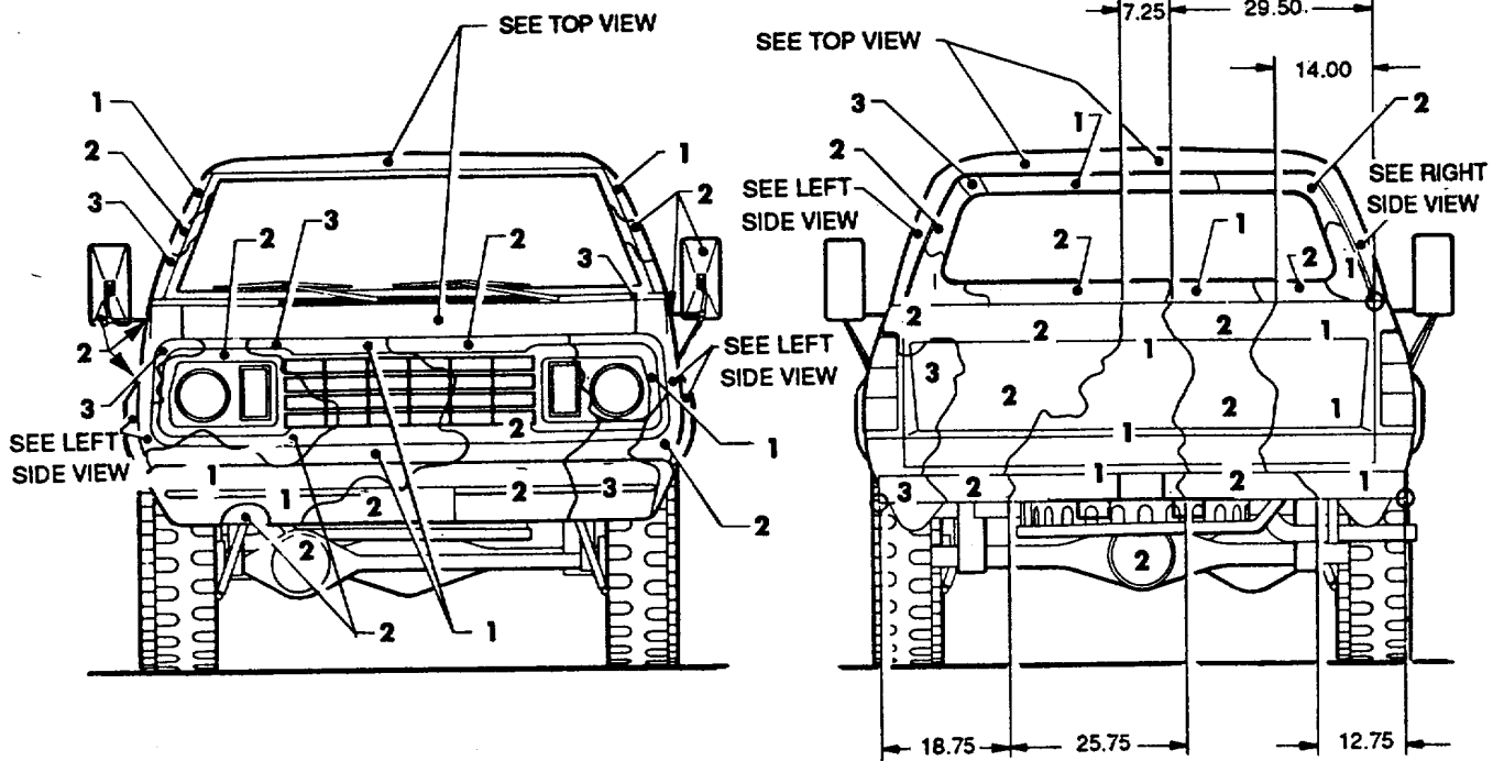
REAR VIEW
