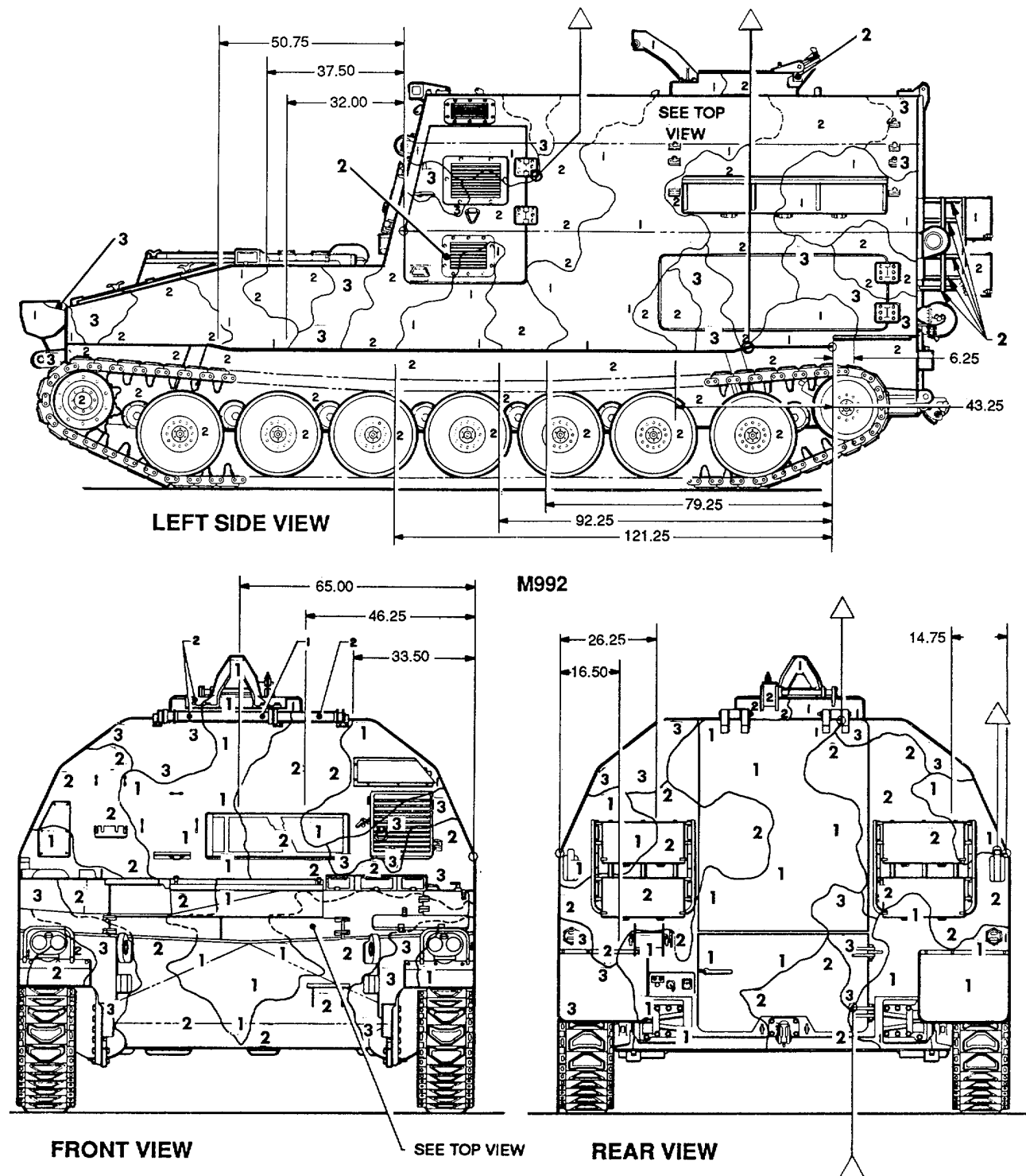
Figure 119. Carrier, ammunition, tracked: M992. (2 of 2)
