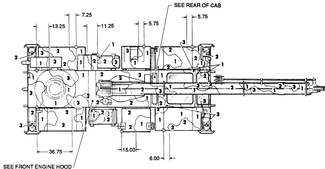
TOP VIEW
