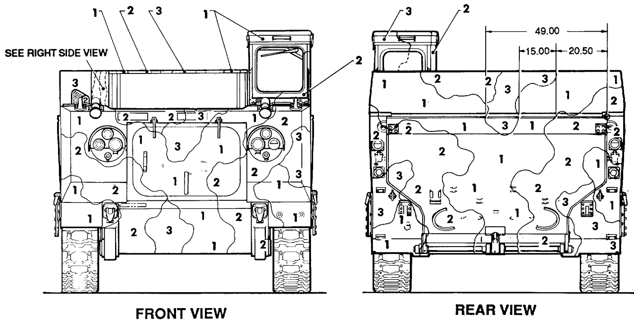
Figure 100. Self-propelled Launcher (SPL) M752, Loader-transporter (LT) M688. (2 of 2)
