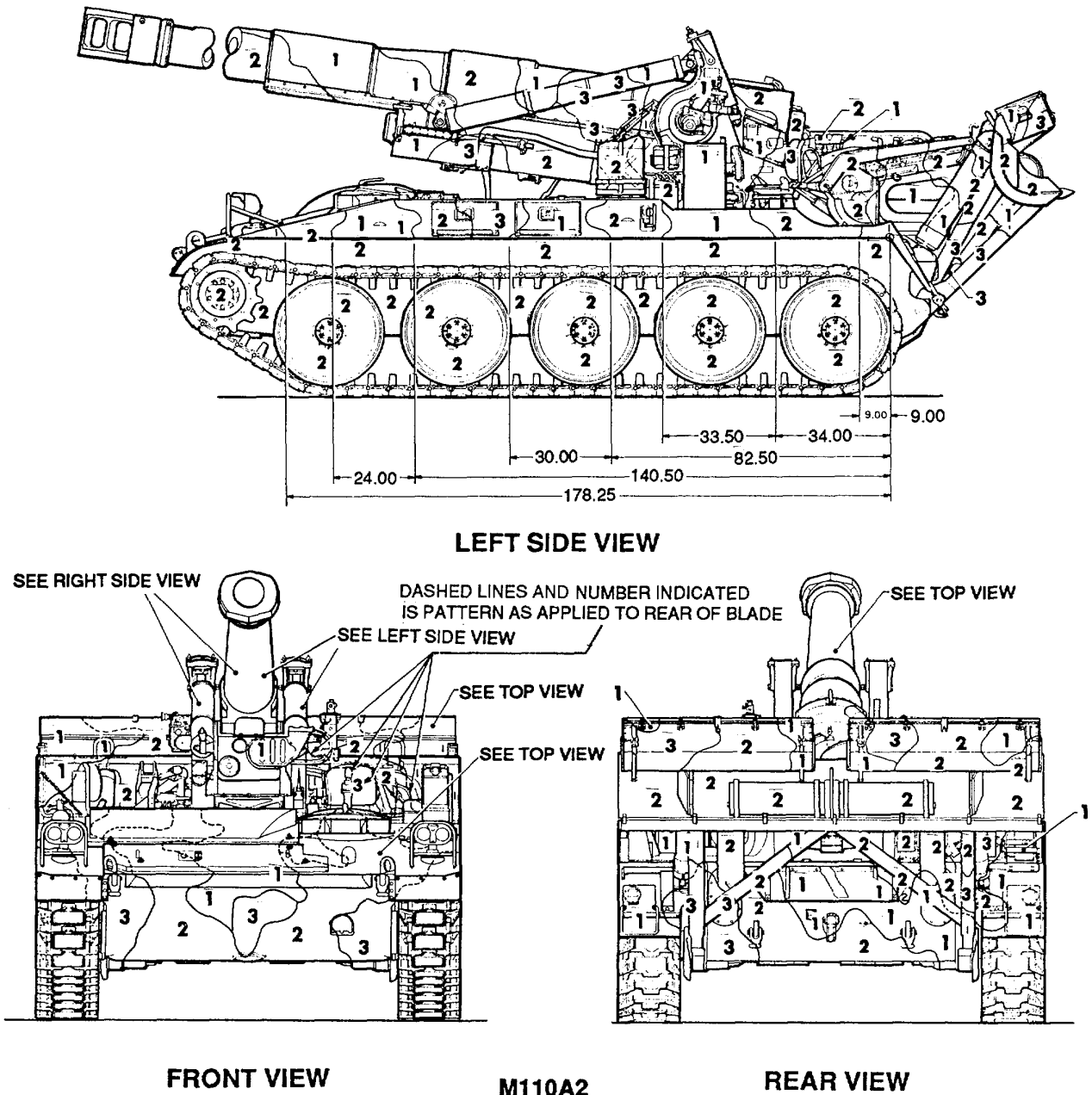
Figure 107. Howitzer, self-propelled: 8-inch, M110A2. (2 of 2)
