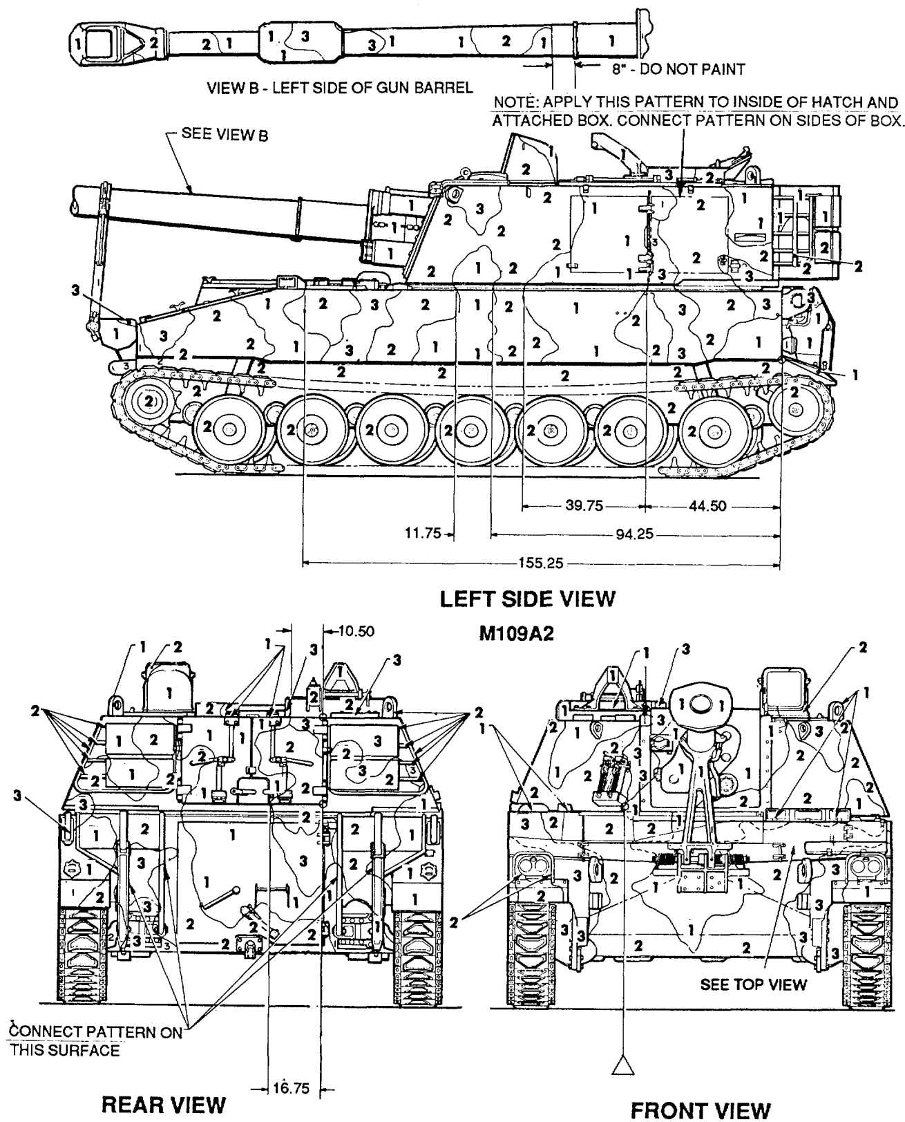
Figure 106. Howitzer, medium, self-propelled: 155-mm, M109A2. (2 of 2)
