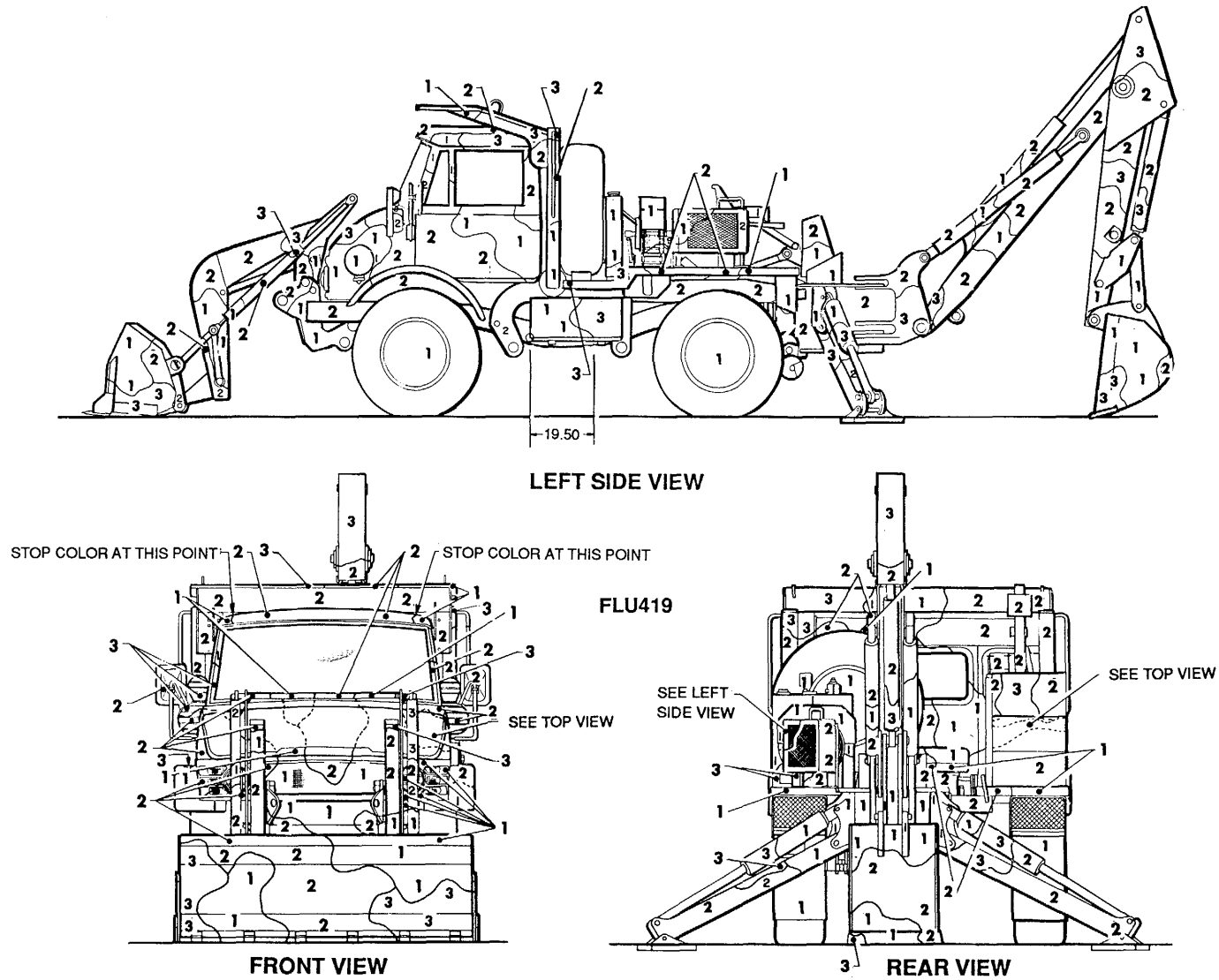
Figure 162. Small emplacement excavator, FLU419. (2 of 2)
