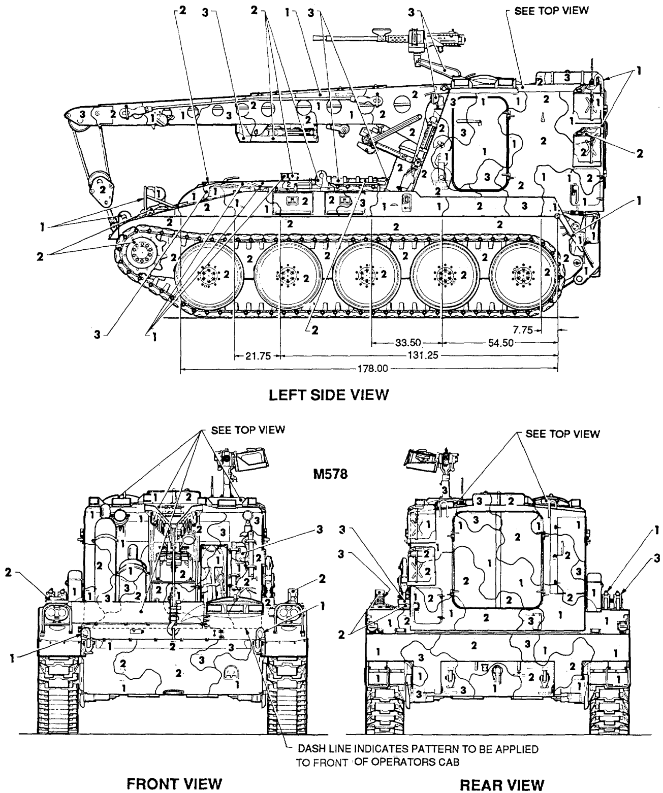
Figure 114. Recovery vehicle, armored: M578. (2 of 2)
